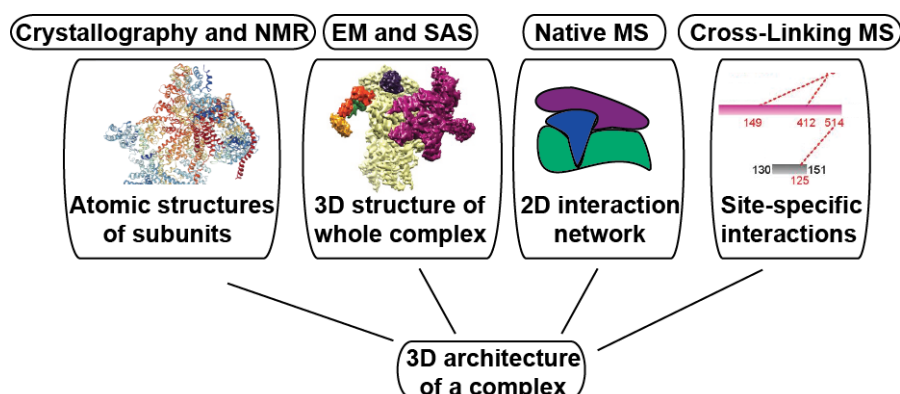
Figure 5. Integrative structural biology. When scientists investigate the structure of dynamic macromolecular assemblies, they require data obtained through a ‘hybrid approach’. They can use distinct methods including high-resolution approaches (such as NMR) and lower-resolution methods such as small-angle X-ray scattering and MS (e.g., cross-linking MS [25] and native MS).
