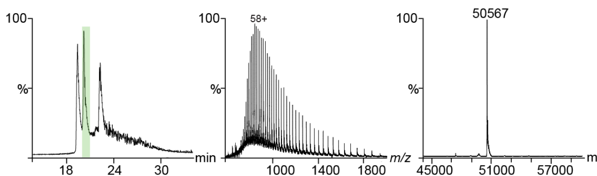
Figure 3. Example of a HPLC-ESI-MS experiment. A trimeric complex (known as the yCAF1 complex [18] ) was analysed by MS under denaturing conditions. Left panel: the three subunits of the complex (i.e., Cac1, Cac2, and Cac3) were chromatographically separated, yielding three distinct retention times (RTs). Central panel: MS spectrum of Cac3 (RT = 20.1 min). Right panel: deconvoluted spectrum of Cac3. The average mass was calculated from the protein sequence (50525 Da). The detected mass (50567 Da) was higher than the expected one; this mass difference indicated the presence of an acetylation mark (42 Da) [10b] .
