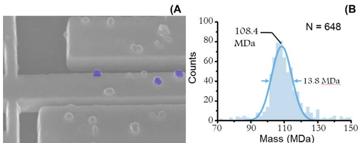
Figure 31. Preliminary NEMS results. (A) Scanning electron microscope image of bacteriophage T5 capsids (blue, false colour) observed on NEMS beam after particle landing and mass sensing. Polymer particles are grey. (B) NEMS-MS spectrum of intact DNA filled T5 capsids.
