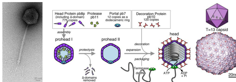
Figure 29. Information about the bacteriophage T5. A) Negative-stain electron microscopy image of phage T5 (diameter of the capsid: 90 nm). B) Scheme of phage T5 head assembly pathway. First, 775 copies of the head protein (i.e., pb8), 12 copies of the portal protein pb7 and unknown number of the head maturation protease pb11 assemble into a pro-capsid ( prohead I ). Then pb11 is activated, it cleaves itself and the N-termini of pb8 and of pb7, yielding an empty prohead II . Finally, the packaging of the 121 kb double-stranded (ds) DNA into prohead II is fuelled by an ATP-dependent molecular motor. The dsDNA packing triggers a two-fold increase of the capsid volume. The expanded mature capsid is then sealed by the head completion protein p144, and decorated with 120 copies of pb10 at the capsid surface.
