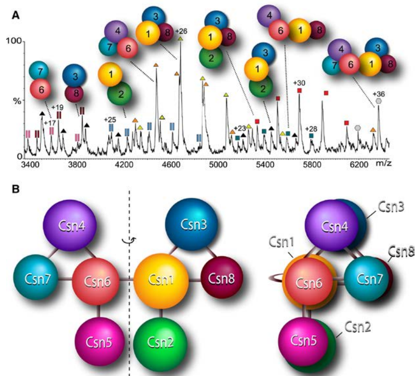
Figure 13. Subunit map of the human CSN Complex. (A) An 3400-6200 m/z range of the mass spectrum recorded when the CSN complex was in absence of the Csn5 subunit. Experimental conditions were optimised to induce the formation of subcomplexes (labeled with the topological arrangement of subunits). In particular, 5%–12.5% methanol (v/v) was added to generate subcomplexes. (B) The protein interaction map of the eight-subunit assembly was determined through the composition of the different subcomplexes. Two distinct modules containing Csn1/2/3/8 and Csn4/5/6/7 were identified. A single interaction between Csn1 and Csn6 could link the two modules. In each module (Csn1/3/8 or Csn4/6/7) each subunit interacted with the other two. On the contrary, the most peripheral subunits, Csn2 and Csn5, bound only a subunit. Figure was from [38] .
