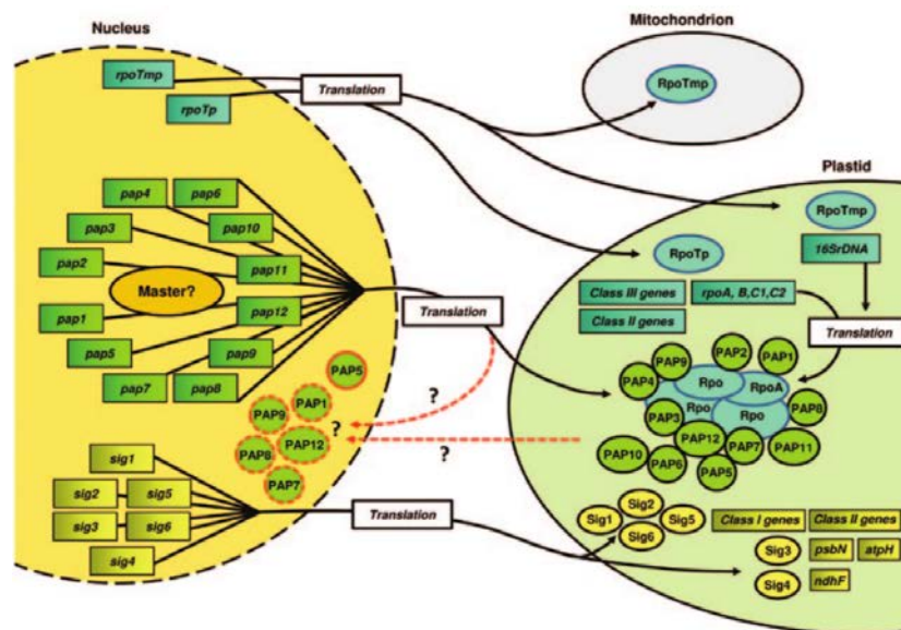
Figure 28. Transport and localization of the PAP proteins and of the composition of the PEP complex.
