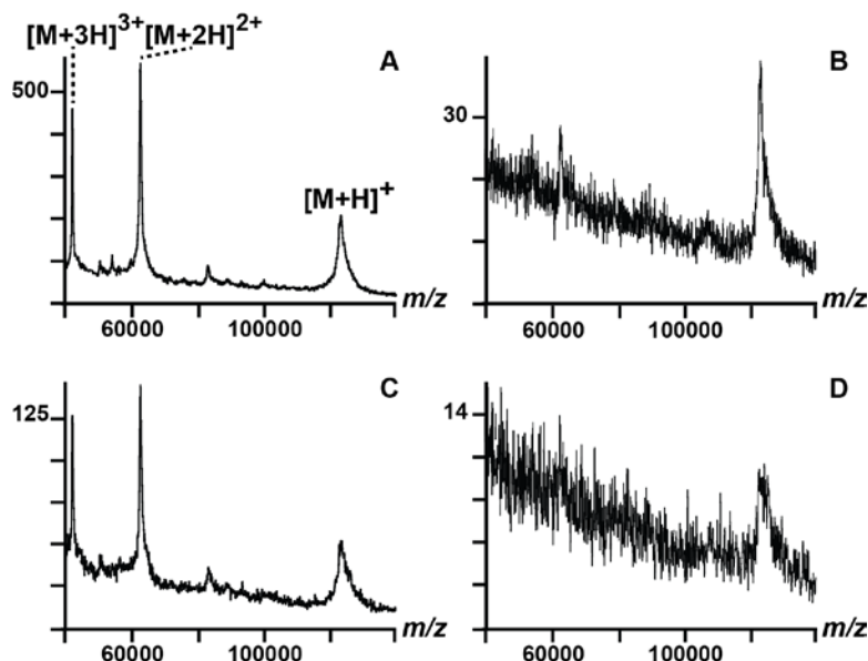
Figure 18. MALDI-TOF analysis of the intact Chromosome region maintenance 1 protein (Crm 1). The molecular weight of this protein is 123386 Da. A) 1 pmole of Crm1 was analysed using the DHB_CHCA mix as matrix. B) amount: 1 pmole; matrix: SA. C) amount:
