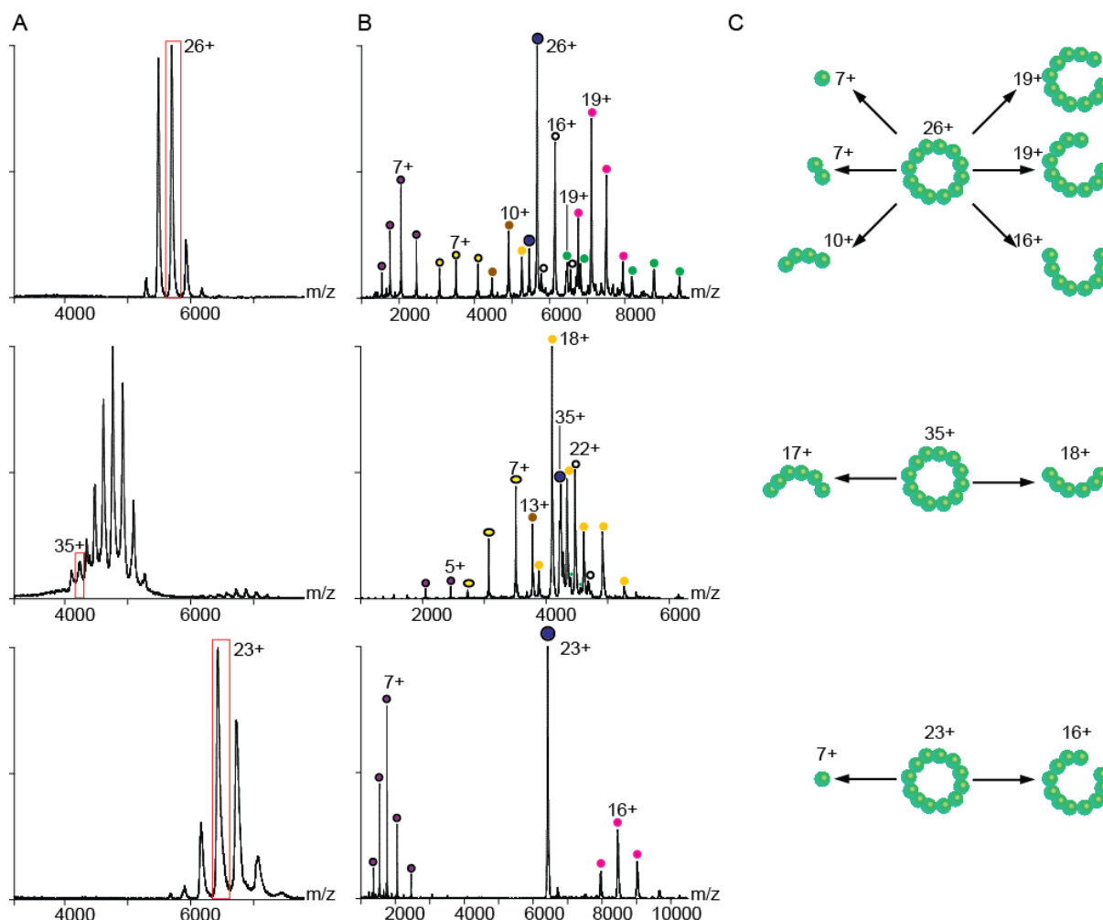
Figure 11. MS and MS/MS spectra of the SP-1 protein complex from different solution conditions. (A) MS spectra of the SP-1 protein complex in three different solution conditions: 100 mM ammonium acetate (top panel), 6.25% sulfolane (middle panel), 2.5% DMSO (lower panel). (B) MS/MS spectra of three charge states of the SP-1 protein complex: 26+ (top panel), 35+ (middle panel), 23+ (lower panel). 12-mer, blue circles; 11-mer, pink circles; 10-mer, green circles; 8-mer, white circles; 6-mer, orange circles; 4-mer, brown circles; 2-mer, yellow ellipses; 1-mer, purple circles. (C) Schematic representations illustrate the dominant dissociation pathways when the SP-1 protein complex is in the three different charge states. The SP-1 26+ ions eject 1-mers, 2-mers, and 4-mers, forming 8-mers, 10-mers, and 11-mers. The SP-1 35+ ion dissociates predominantly via the formation of 6-mers. The SP-1 23+ ion ejects 1-mers, generating 11-mers. Figure from [36] .
