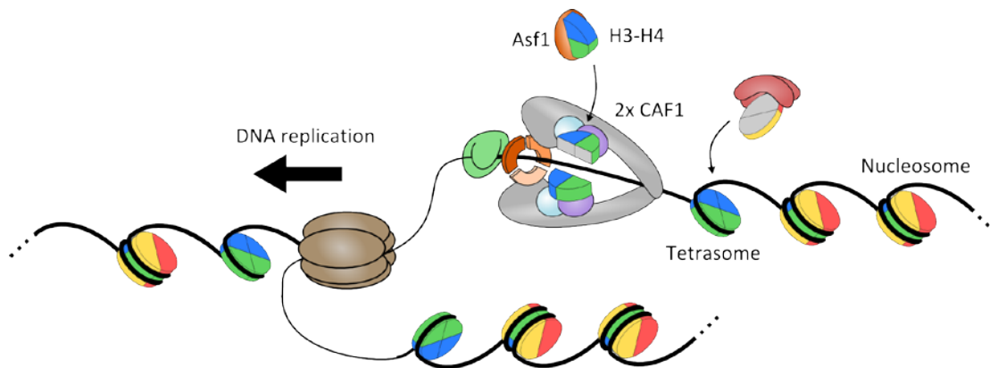
Figure 17. Model for yCAF1 recruitment and H3-H4 deposition. A yCAF1 complex (labelled in grey, light blue and violet) is loaded with dimeric H3-H4 through association of yAsf1. Two yCAF1-H3-H4 complexes bind cooperatively to an extended DNA sequence and deposit two H3-H4 dimers and form tetrasomes. Additional proteins (such as the one labelled in orange) are required for deposition of H3-H4 tetramers. Then, H2A-H2B chaperones recognise the H3-H4 tetrasome and deposit two copies of H2A-H2B to form a complete nucleosome (i.e., 2 H2A, 2 H2B, 2 H3 and 2 H4).
