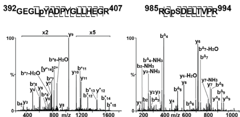
Figure 7. Spectra of in vivo phosphorylated p140 peptides. The protein p140 was immunoprecipitated from human cells, proteolysed and then its peptides were analysed by LC-MS. Each peptide was fragmented inside the mass spectrometer in order to allocate the position of the phosphorylated sites [31].
