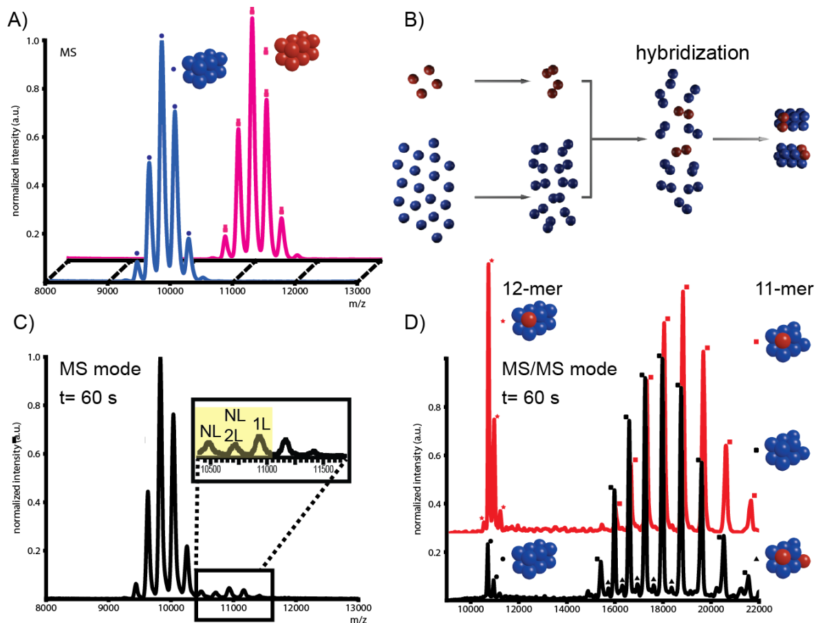
Figure 20. Self-assembly mechanism of TET2. A) MS spectra of the non-labelled (NL) TET2 12-mer (blue) and the [ ^{15}\text{N} , ^{13}\text{C} , ^2\text{H} ] fully labelled (L) (red) TET2. The signals of the NL and L dodecamers (12-mers) do not overlap due to a significant mass difference. B) To do “isotopic hybridization” experiments we utilised NL and L 1-mers (i.e., disassembled complexes) as starting material. 60 seconds after the beginning of the self-assembly reaction, the NL and L were mixed. In this way, L intermediates were incorporated into final “isotopically hybrid” complexes which were further analysed by tandem MS. C) A MS spectrum of an isotopically hybrid 12-mer. D) Tandem MS spectra of two isotopically hybrid TET2 12-mers whose m/z were 10700 and 10900, respectively.
