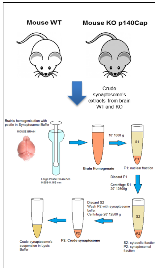
Figure 8. Workflow to characterise the p140Cap synaptic interactome. We analysed the p140Cap synaptic interactome using co-immunoprecipitation from crude mouse synaptosomes and MS-based proteomics. We identified 351 p140Cap interactors and found that they cluster to subcomplexes mostly located in the postsynaptic density (PSD). Figure from [34].
