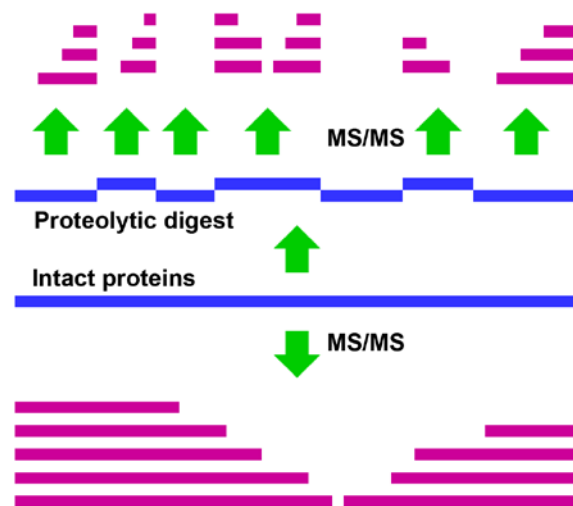
Figure 1. Analysis of proteins by MS. In bottom-up proteomics (top), proteins are proteolysed using an enzyme (such as trypsin), and the resulting peptides are analysed in two stages. In the first stage (known as “MS mode”), the masses of the intact tryptic peptides are determined. In the second stage (aka “MS/MS mode” or “tandem MS mode”), these peptide ions are further fragmented to obtain information about the sequence of the digested proteins and their post-translational modifications (PTMs). Using the top-down approach (bottom), intact protein ions are fragmented in the mass spectrometer. This provides the molecular mass of the proteins and of their fragment ions. Figure was adapted from [3] and Wikipedia.
