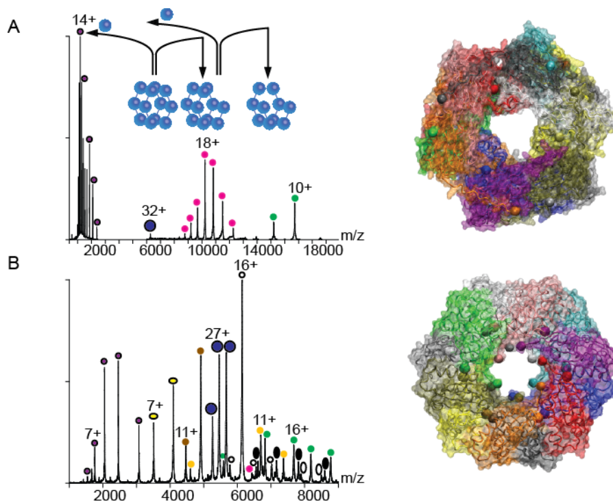
Figure 10. Features of the HSP16.9 and SP-1 macromolecular assemblies. (A) The HSP16.9 protein complex. Left panel: MS/MS spectrum of intact dodecameric (12-meric) HSP16.9 32+ ions. A schematic representation illustrates how this protein complex dissociates by forming lowly charged decamers (10-mers) and undecamers (11-mers) at high m/z and highly charged monomers at low m/z . This type of dissociation is defined as “typical” because there is sequential loss of monomeric (1-meric) subunits. 12-mer: blue; 11-mer: pink; 10-mer: green; and 1-mer: purple. Right panel: Crystal structure of the HSP16.9 protein complex (PDB code: 1gme). The N- and C-terminal amino acids of each protein within the protein complex are represented as spheres in order to clearly illustrate their positions. The N-termini of chains B, D, F, H, J, and L are disordered and not present in the crystal structure. (B) The SP-1 protein complex. Left panel: MS/MS spectrum of intact 12-meric SP-1 27+ ions. 1-mers, 2-mers, 3-mers, 4-mers, 5-mers and 11-mers, 10-mers, 9-mers, 8-mers, 7-mers, 6-mers are present at low and high m/z in the spectrum, respectively. The dissociation of SP-1 is “atypical” due the ejection of dimers (2-mers) and tetramers (4-mers). 12-mer, blue circles; 11-mer, pink circles; 10-mer, green circles; 9-mer, white ellipses; 8-mer, white circles; 7-mer, black ellipses; 6-mer, orange circles; 4-mer, brown circles; 2-mer, yellow ellipses; 1-mer, purple circles. Right panel: The crystal structure of the SP-1 protein complex (PDB code: 1tr0). Figure from [36] .
