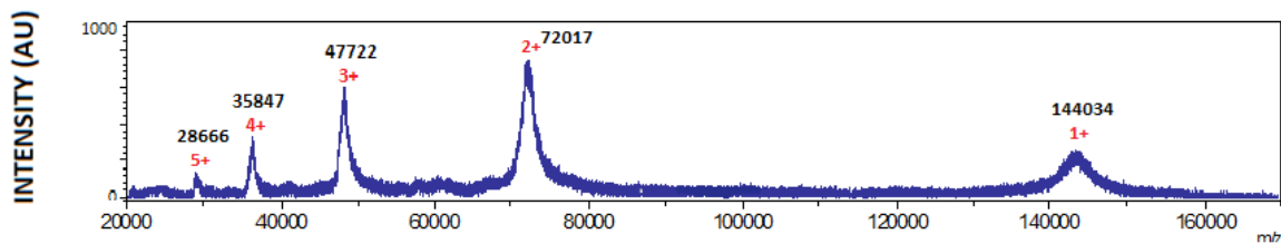
Figure 25. An intact Ab was analysed by MALDI-TOF. This analysis generated Ab peaks with five distinct charge states ranging from 1+ to 5+. The MALDI-TOF approach is sensitive because a picomole of sample is sufficient for a successful analysis. However, the resolution is suboptimal. Moreover, it is difficult to assess the charge of the species and not all the peaks could be assigned with high confidence. Therefore, ESI-MS complements the MALDI-based approach.
