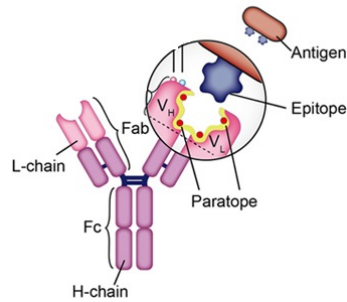
Figure 27. Schematic representation of the interactions between epitope and paratope. Figure adapted from Creative Diagnostics.
