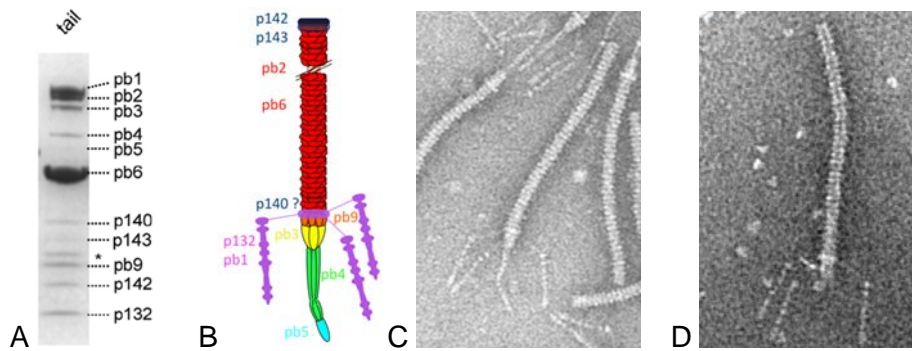
Figure 30. Tail of phage T5. A) Subunits forming the tail were analysed by SDS-gel electrophoresis. The eleven proteins have the following expected masses. Pb1, 148 kDa; pb2, 121.9 kDa; pb3, 107.3 kDa; pb4, 74.9 kDa; pb5, 67.8 kDa; pb6, 50.3 kDa; p140, 34.5 kDa; p143, 27.8 kDa; p9, 22.7 kDa; p142, 18.4 kDa; p132, 15 kDa [63c] . B) Schematic representation of T5 tail [63c] . C) and D) negative stain EM images of T5 tail before (C) and after (D) its interaction with FhuA. The tip of the tail seems to disappear, and it is unknown whether some of the T5 proteins may dissociate from the tail. Diameter of the tail tube: 10 nm.
