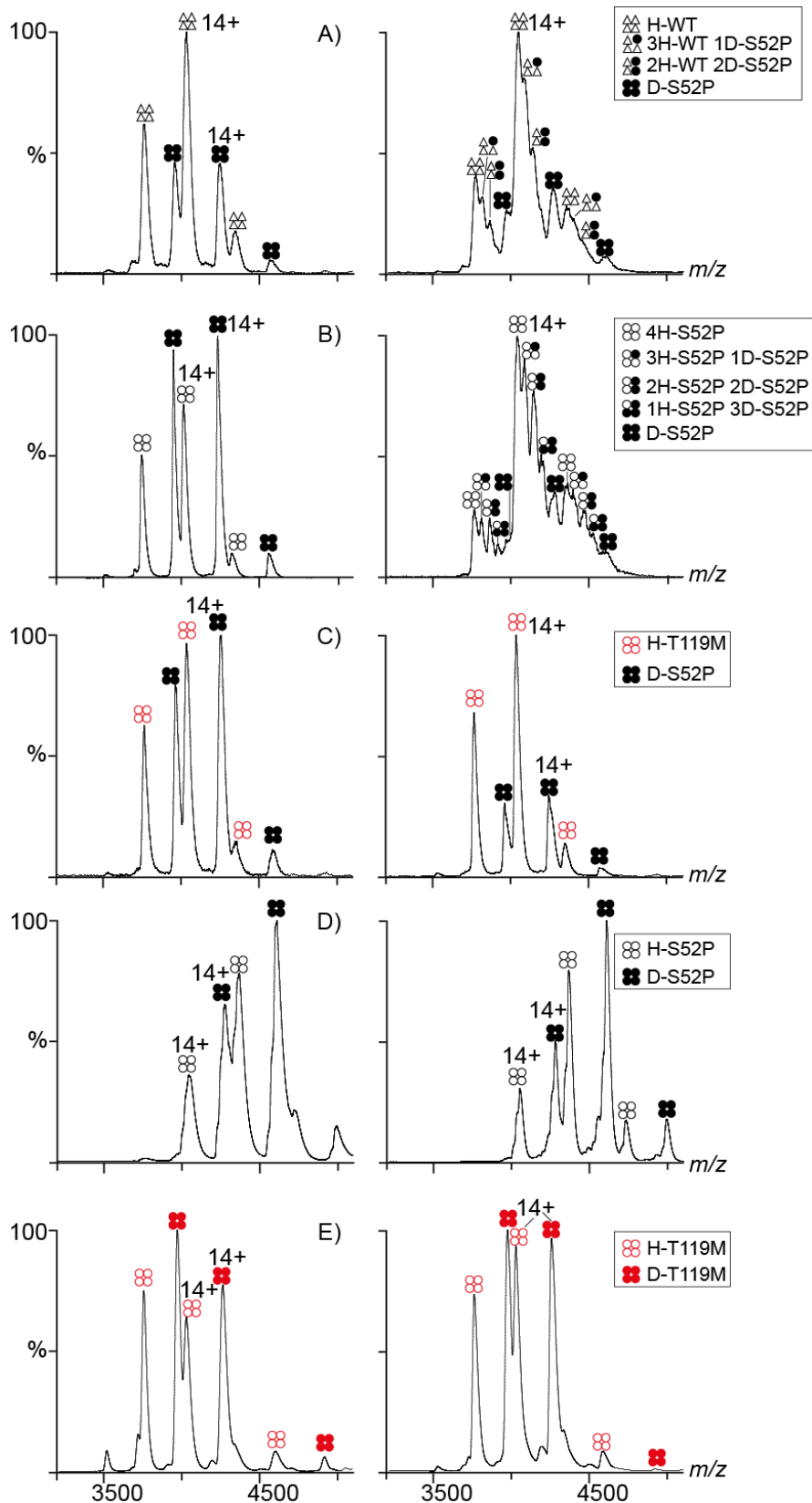
Figure 15. MS spectra of the subunit exchange of TTR. Reactions between deuterated S52P and hydrogenated (A) WT, (B) S52P, (C) T119M, and (D) S52P bound to tafamidis, were monitored. The shown spectra were recorded at the beginning of the reaction (left
