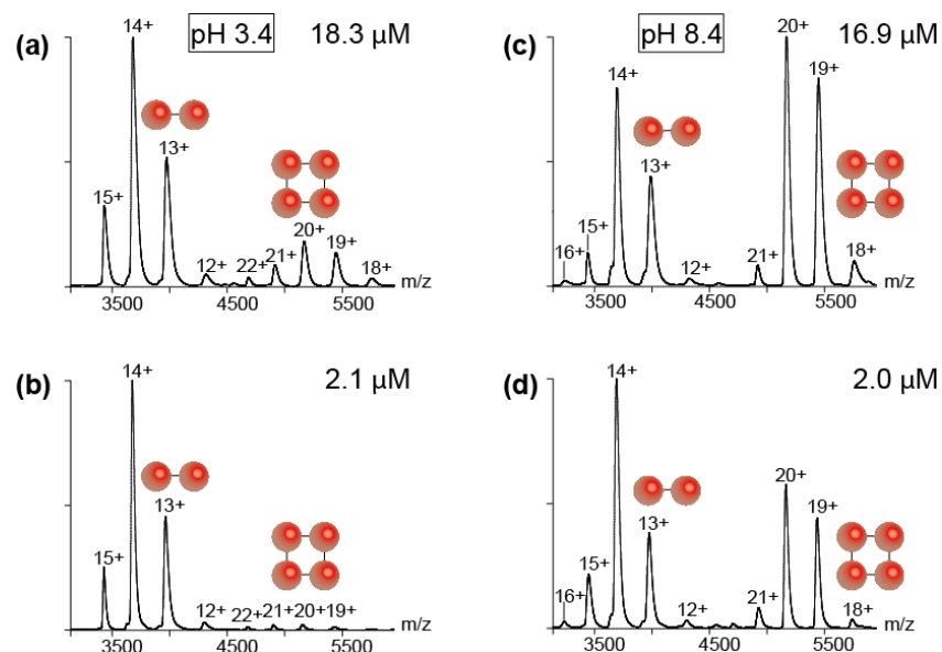
Figure 12. Relative abundance of dimers and tetramers versus solution concentration of concanavalin A. The solution pH highly influences the oligomeric state of concanavalin A. (a) Spectrum of intact concanavalin A at D_0 = 18.3 \mu\text{M} and pH 3.4; (b) spectrum at D_0 = 2.1 \mu\text{M} and pH 3.4; (c) spectrum of concanavalin A at D_0 = 16.9 \mu\text{M} and pH 8.4; (d) spectrum of concanavalin A at D_0 = 2.0 \mu\text{M} and pH 8.4. Two spheres indicate the dimeric ions and four spheres indicate tetrameric ions. Figure from [15] .
