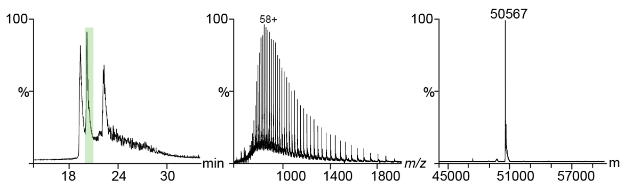
Figure 3. Example of a HPLC-ESI-MS experiment. A trimeric complex (known as the yCAF1 complex [18]) was analysed by MS under denaturing conditions. Left panel: the three subunits of the complex (i.e., Cac1, Cac2, and Cac3) were chromatographically separated, yielding three distinct retention times (RTs). Central panel: MS spectrum of Cac3 (RT = 20.1 min). Right panel: deconvoluted spectrum of Cac3. The average mass was calculated from the protein sequence (50525 Da). The detected mass (50567 Da) was higher than the expected one; this mass difference indicated the presence of an acetylation mark (42 Da) [10b].
