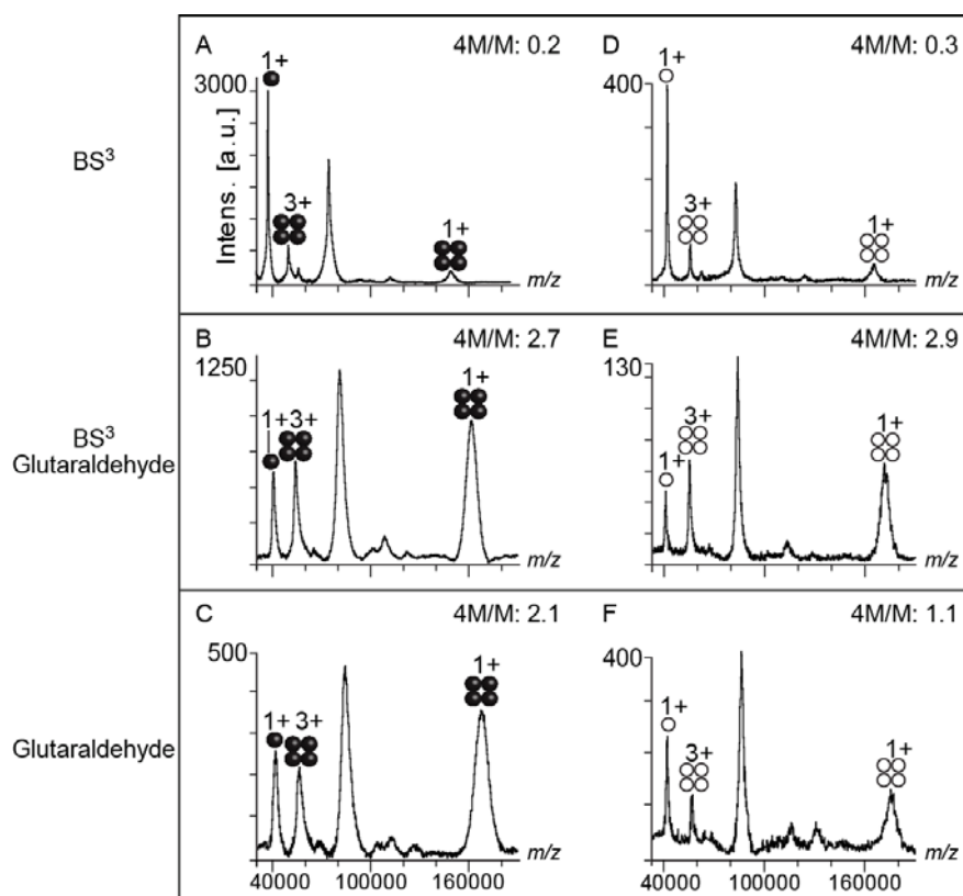
Figure 19. Combining two XLers using gentle agitation in a thermomixer at pH 7.2. We XLed the ADH using A) BS 3 alone, C) glutaraldehyde alone or B) a combination of the two reagents. The aldolase was XLed utilizing D) BS 3 , F) glutaraldehyde or E) both. The ADH and aldolase subunits are labeled as black and white spheres, respectively. The ratio 4M/M is a semi-quantitative indicator of XLing efficiency. Four spheres show the tetrameric peaks. The ratio 4M/M is the sum of the intensities of the tetrameric ions (i.e. [4M+ H] 1+ and [4M+
