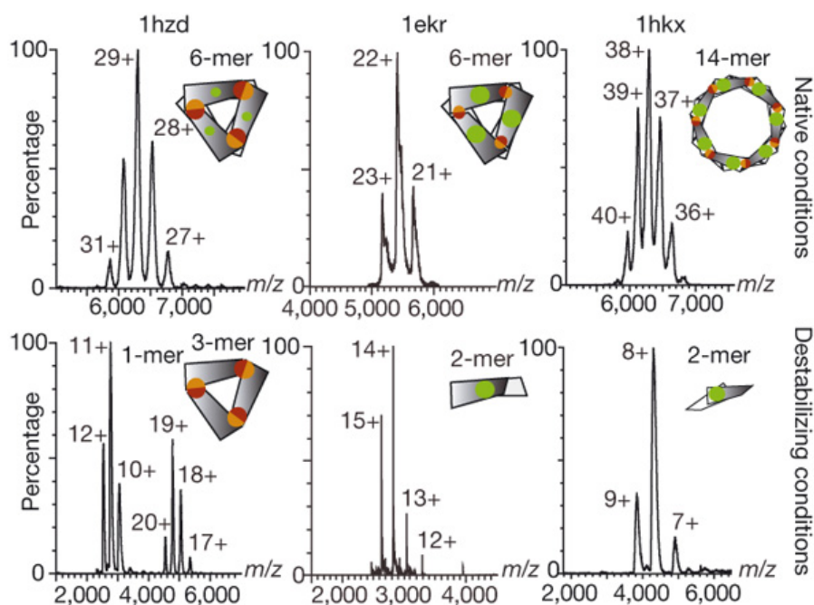
Figure 9. Native mass spectra of intact complexes (top panel) and of subcomplexes obtained after destabilisation in solution (bottom panel). These complexes were previously crystallised. Using destabilisation conditions I was able to selectively break the weakest interactions and preserve the strongest interactions. This means that the building blocks were isolated by native MS. My results were consistent with crystallographic data present in the PDB database. 1hzd: AUH, an RNA binding protein; 1ekr: molybdenum cofactor biosynthesis protein; 1hcx: Ca 2+ /calmodulin-dependent kinase II [13] .
