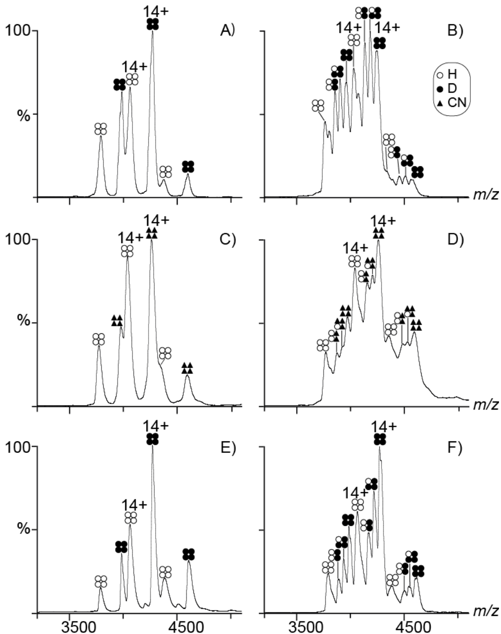
Figure 14. Native MS spectra of mixed unlabeled and isotope-labeled WT-TTR. A) 38 minutes after mixing H-TTR (unlabelled protein) and D-TTR (labelled). In the spectrum six peaks are present matching the masses of the 4H and 4D TTR homo-tetramers. B) TTR spectrum after 8 days of the H-TTR and D-TTR mixing. C) TTR spectrum 7 minutes after mixing 4H and 4CN (TTR labelled with ^{13}\text{C} ^{15}\text{N} isotopes). D) The same reaction was monitored after 10 days. H-ammonium acetate was used for the samples shown in A–D. E) 7 minutes after mixing H-TTR and D-TTR. F) TTR spectrum after 8.8 days of mixing H-TTR and D-TTR. D-ammonium acetate dissolved in \text{D}_2\text{O} was used for the samples in (E) and (F).
