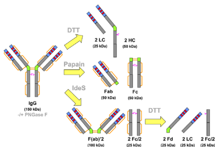
Figure 24. Abs can be characterised using MS according to a “middle-down” approach [55] . Abs are analysed intact before and after deglycosylation treatment using the enzyme PNGase. Abs are also investigated as fragments generated after enzymatic digestion and/or after disulfide bridge reduction. Adapted from [47] .
