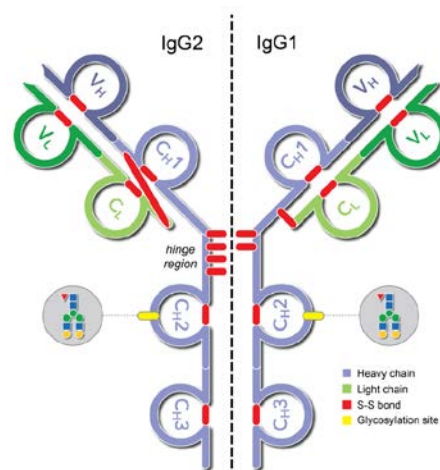
Figure 22. IgG structure. Adapted from [50]
