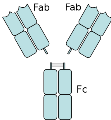
Figure 23. An antibody proteolysed by papain. It yields three fragments: two Fab fragments and one Fc fragment. Adapted from Wikipedia.
