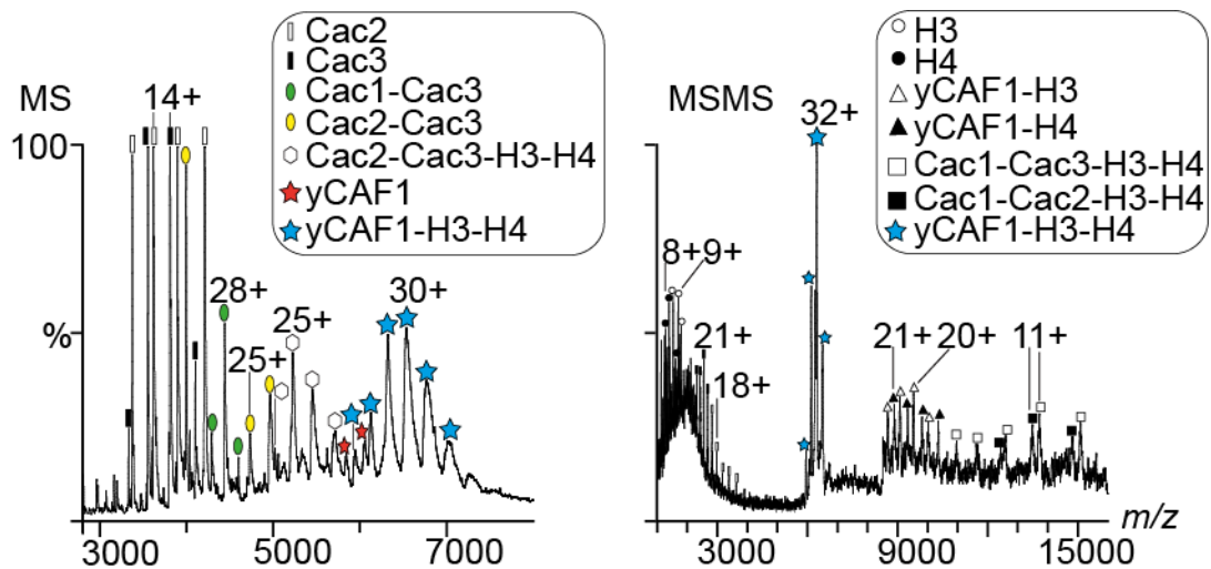
Figure 16. MS and MS/MS spectra of the yCAF1-H3-H4. Left panel: MS spectrum of the heteroassembly. In addition to the intact CAF1, trimer in the unbound state (174 kDa) and bound to H3-H4 (201 kDa) (labeled as red and cyan stars, respectively), dimers such as Cac1-Cac3 (green ellipses) and Cac2-Cac3 (yellow ellipses), trimers such as Cac2-Cac3-H3-H4 (white hexagon), and single monomeric proteins (blank and white rectangles) were also detected. Most likely, these subcomplexes were present in solution and not generated in the gas phase. Right panel: MS/MS spectrum of the 32+ ions confirmed a 1:1:1:1 stoichiometry of the yCAF1-H3-H4 complex. Figure from [18] .
