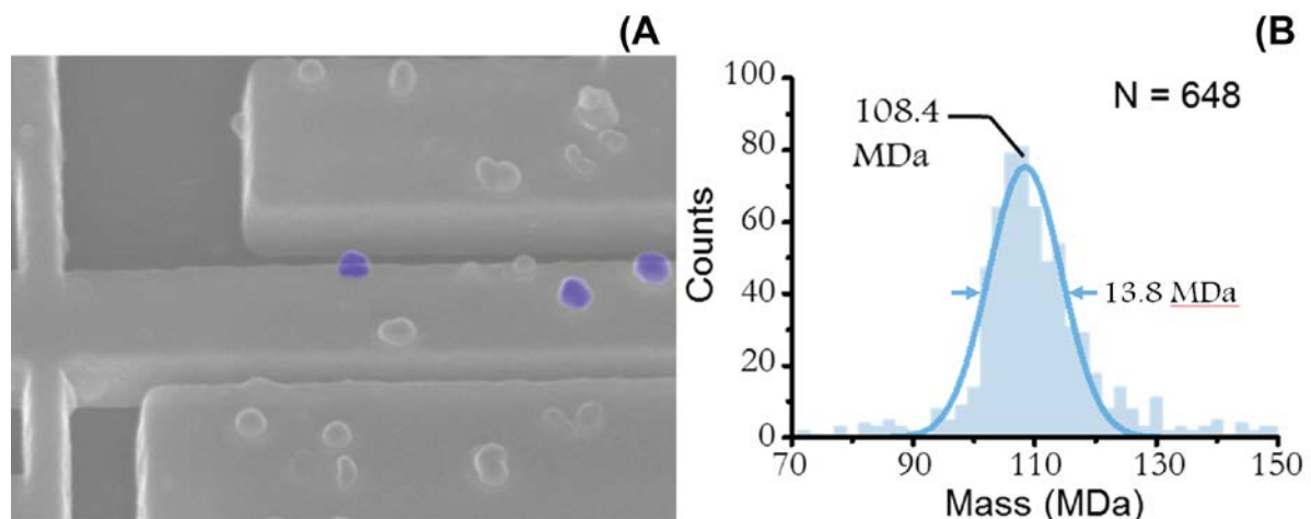
Figure 31. Preliminary NEMS results. (A) Scanning electron microscope image of bacteriophage T5 capsids (blue, false colour) observed on NEMS beam after particle landing and mass sensing. Polymer particles are grey. (B) NEMS-MS spectrum of intact DNA filled T5 capsids.
