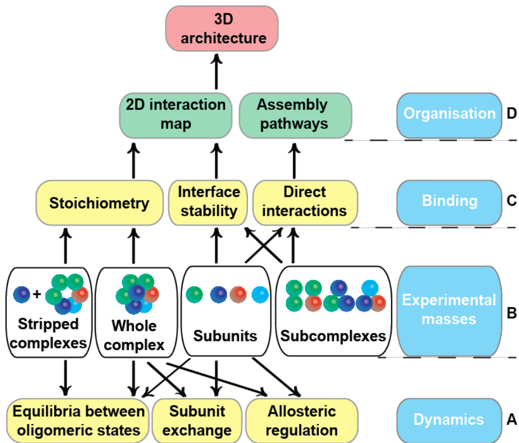
Figure 2. Native MS provides diverse information about macromolecular complexes.
