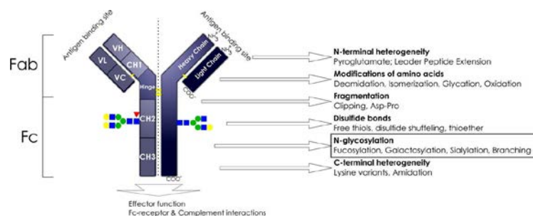
Figure 26. Possible modifications and alterations of an IgG. Figure adapted from [49a]
