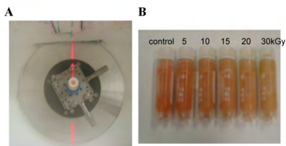
Figure 3: (A) Sample environment on ID17 beamline at ESRF. (B) 2 ml samples of D. radiodurans cells following irradiation with 0, 5, 10, 15, 20 and 30 kGy. The pink colour of D. radiodurans cells is due to the presence of deinoxanthin (a carotenoid). Irradiation of the cells significantly alters the colour of the cells.
