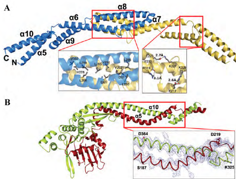
Figure 19: (A) Crystal structure of the dimeric coiled-coil domain of RecN. A close-up view of the dimer interface is shown in the box. Residues involved in dimerisation are represented as sticks. Distances are reported for intermolecular ionic interactions that stabilise the anti-parallel fold of the coiled-coil. (B) Crystal structure of RecN \Delta dd in which the N-terminal region is coloured red and the C-terminal domain is coloured light green. Helices \alpha 5 and \alpha 10 are respectively \sim 75 and \sim 100 Å long and present large kinks that determine the orientation of the coiled-coil domain. A close-up view of the final electron density map (2Fo-FC map contoured at 1.5\sigma ) is shown for the central region of the coiled-coil, which allowed us to obtain a full model of helices \alpha 5 and \alpha 10 that were only partially visible in our RecNHead and RecNcc structures.
