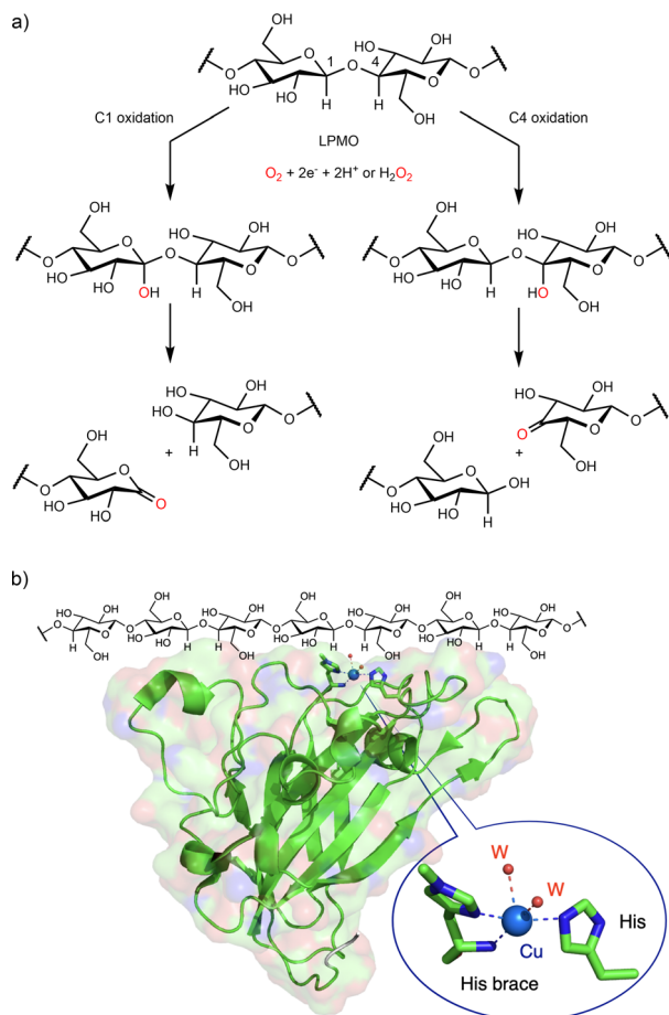
Fig. 4 Lytic polysaccharide monoxygenase (LPMO). (a) Reactions catalyzed by LPMO; (b) LPMO X-ray structure from Thermoascus aurantiacus (PDB ID 2ye2) showing the copper active site at the binding surface of the LPMO.
