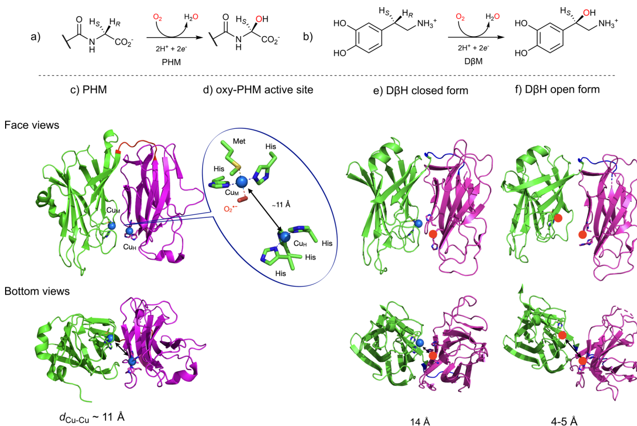
Fig. 2 Uncoupled binuclear copper-containing monooxygenases, PHM and D \beta H. (a) and (b) reactions catalyzed by PHM and D \beta H, respectively; (c) X-ray structure of PHM from Rattus norvegicus showing the two domains (Cu M domain in green and Cu H domain in magenta) connected by a loop (in blue) in which each domain binds a single copper atom spaced from each other by approximately 11 \text{\AA} and (d) structure of the Cu M -superoxido intermediate in PHM (PDB ID 1opm); (e) and (f) X-ray structure of the human D \beta H (PDB ID 4zel) showing the open (e) and the closed (f) forms. Only the Cu M domain of the closed form contains a copper atom, the other copper ions (red sphere) are manually placed.
