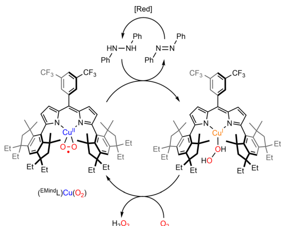
Scheme 7 Reaction of [(^{\text{EMind}}\text{L})\text{Cu}^{\text{II}}(\text{O}_2)] with 1,2-diphenylhydrazine to produce azoarene and [(^{\text{EMind}}\text{L})\text{Cu}^{\text{I}}(\text{H}_2\text{O}_2)] . Adapted from ref. 83.
