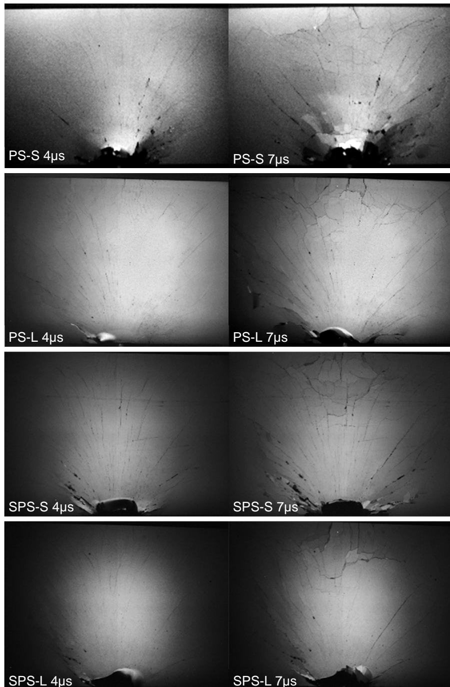
Fig. 8 Images at t = 4 and 7 \mu s of EOI tests performed with 4 SiC ceramics. The striking velocity is 181, 169, 170, 172 m/s for PS-S, PS-L, SPS-S, SPS-L targets, respectively (Forquin et al. 2018)
