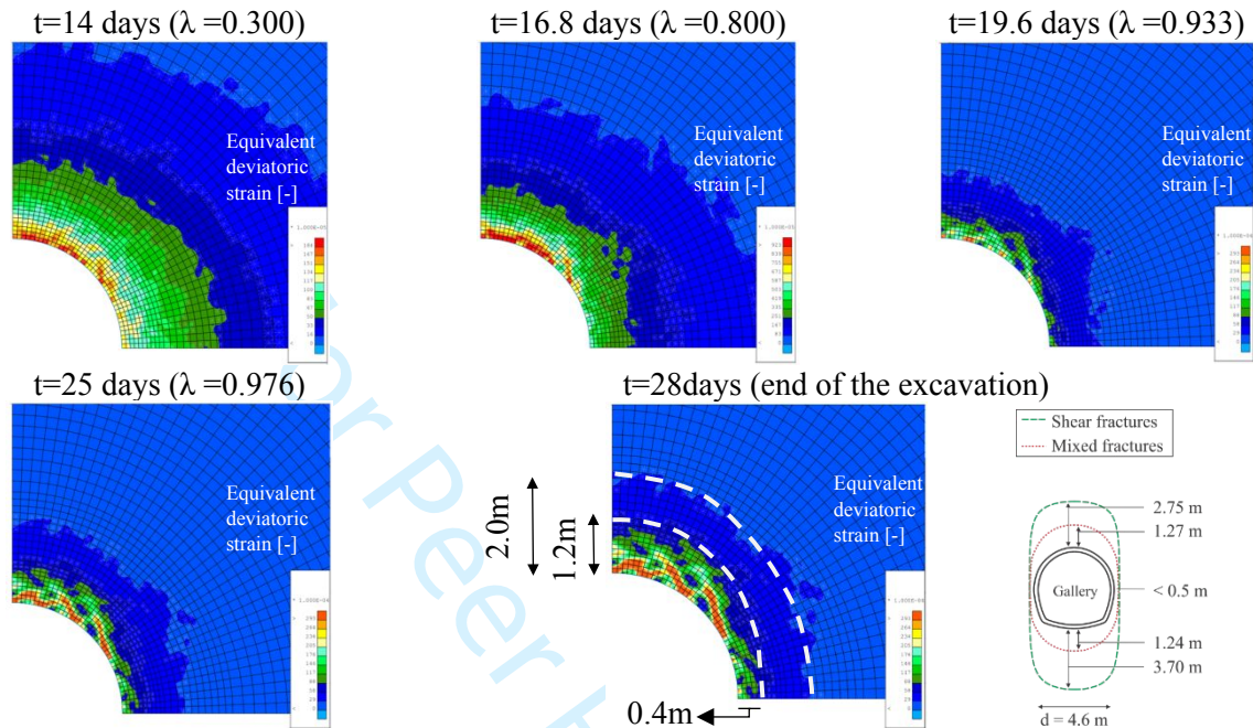
6 7 8 9 Figure 30. Evolution of strain localisation pattern during the gallery excavation using the 50REA_1, 50REA_2, 50REA_4, and 50REA_5 mesostructures with random distribution (equally in proportion) and comparison with experimental fracture measurements 6,46 .
