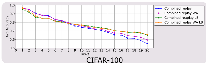
Fig. 11 Final average accuracy of the Combined replay in the CIFAR-100 dataset when using a memory buffer size of 2000 examples.
