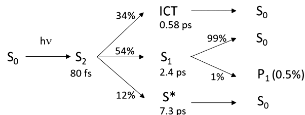
Scheme 2. Picosecond Photodynamics of Synechocystis N-Tagged ECN-OCP upon 540 nm Excitation (Yields Are Estimated from GSB Recovery of OCP O at 490 nm and P_1 Represents Overall Formation Yield from S_2 , Table 1)
