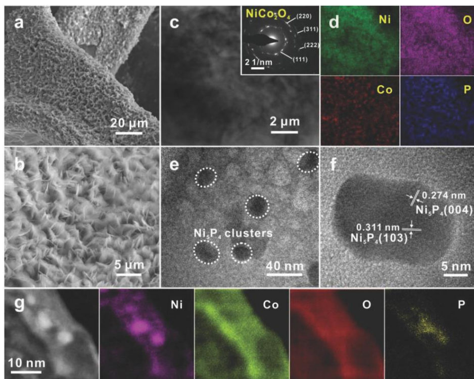
3175 Figure 73. a) SEM image showing the uniformly distributed Ni 5 P 4 @NiCo 2 O 4 nanoflakes on graphene/Ni foam. b) High-magnification SEM image of Ni 5 P 4 @NiCo 2 O 4 nanoflakes. c) Low-magnification TEM image and d) corresponding energy dispersive spectroscopy (EDS) elemental mapping images of Ni 5 P 4 @NiCo 2 O 4 nanoflakes. e) High-resolution TEM image showing that nanometric Ni 5 P 4 clusters are nested on the nanoflakes. f) HRTEM image of one single Ni 5 P 4 nanocluster. g) HRTEM image and corresponding elemental mapping images of Ni 5 P 4 @NiCo 2 O 4 . Reproduced with permission from ref. 1112 Copyright Wiley 2018. 3180
