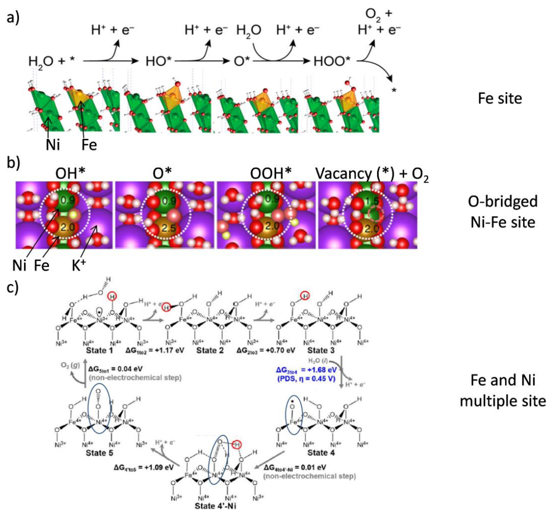
Figure 52. NiFe (oxy)hydroxide active site and OER mechanism by DFT calculations. a) Proposed OER pathway involving the HO * , O * and HOO * intermediates and with a Fe atom site that was substituted in the (0112) surface of \gamma -NiOOH as the active site. Reproduced with permission from ref. 878. American Chemical Society. b) A second proposed OER mechanism and intermediates on the H-saturated O-bridged Ni-Fe site as active site at the (01-10) surface of \gamma -NiFe LDH. The reaction centers are highlighted by large dotted white circles, the vacancy by a small pink dashed circle. The magnetic moments of Ni and Fe during OER are also given. Reproduced with permission from ref. 1775. Copyright Nature Publishing 2020., c) A third example of proposed mechanism for OER on Ni 1-x Fe x OOH catalyst. Blue ovals highlight the
