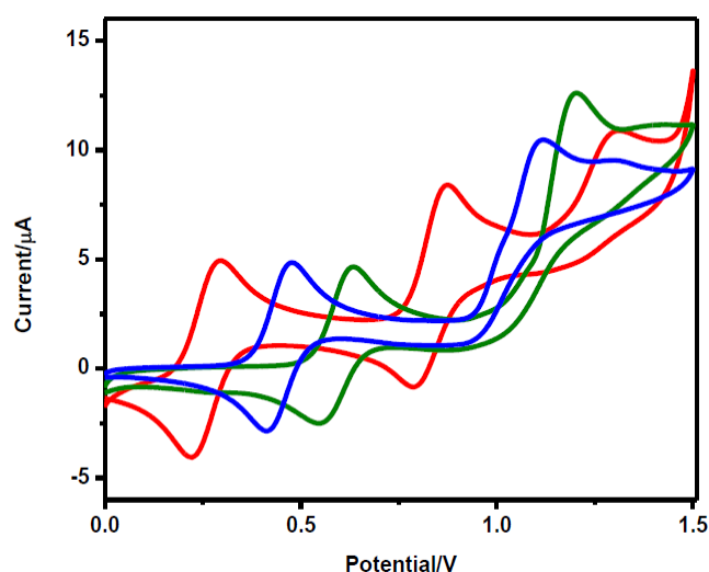
4940 4945 Figure 131. Water oxidation in the presence of Co(tpc)Py 2 (red), Co(tdfc)Py 2 (blue) and Co(tpfc)Py 2 (green) in acetonitrile on adding 4.8% water. Reprinted with permission from Ref. 1577 Copyright 2020. American Chemical Society.
