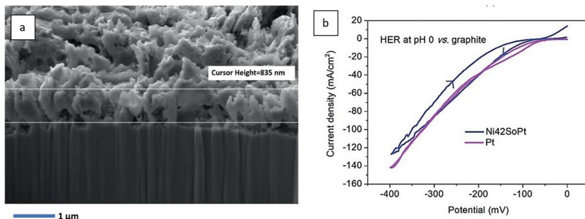
Figure 106. (a) SEM photograph showing the cross-section of the Ni 42 /Pt interface (Pt thickness ~ 800–900 nm); the Pt loading is 1.8 mg/cm 2 . (b) comparison of the HER performances of Pt and Ni 42 SoPt at pH = 0. Reproduced with permission from ref. 1269. Copyright Wiley 2019.
