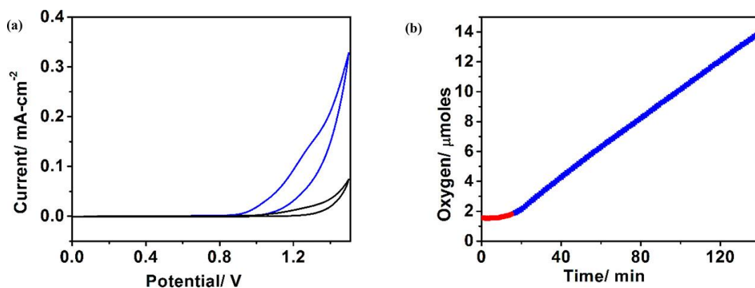
Figure 128. Cyclic voltammograms (V vs Ag/AgCl) of Nafion films, loaded (blue trace) and not loaded (black trace) with \text{Fe}(\text{tpfc})\text{Cl} , on FTO electrodes in pH 10 phosphate–KOH buffer (scan rate of 100 \text{ mV s}^{-1} ; catalyst loading 1.6 \text{ nmol cm}^{-2} ). (b) Evolution of oxygen before (red) and after (blue) application of a potential of 1.5 V. Reprinted with permission from Ref. 1577 Copyright 2020. American Chemical Society.
