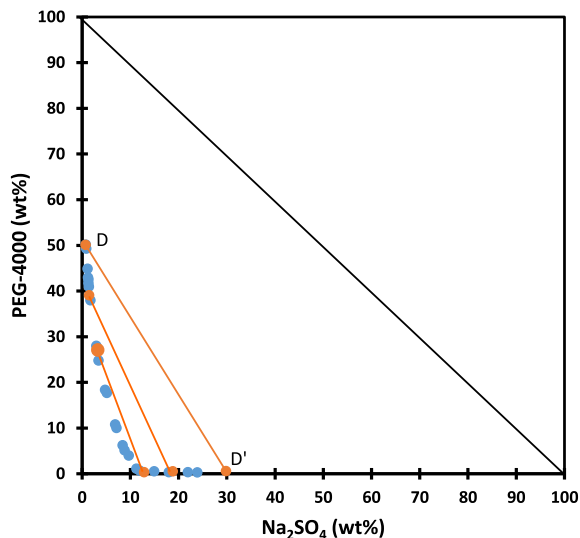
Figure 3. Binodal (blue symbols) and some tie-lines (orange symbols and lines) of the system \text{H}_2\text{O}/\text{Na}_2\text{SO}_4/\text{PEG-4000} at T = 25^\circ\text{C} . Data re-drawn from Ref. [92].
