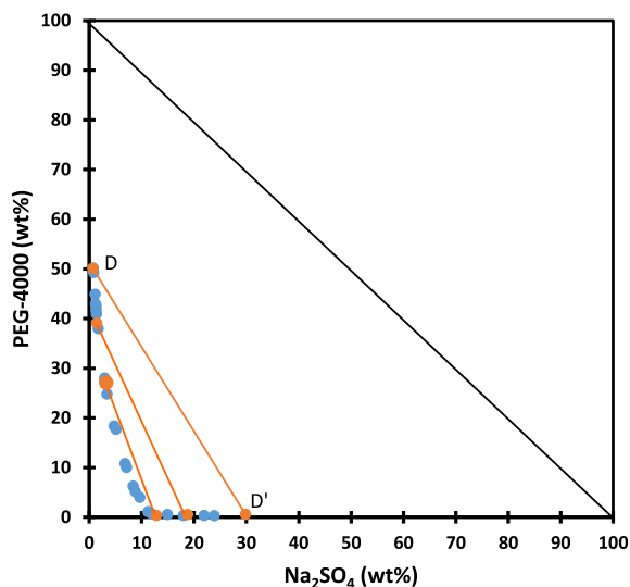
Figure 3. Binodal (blue symbols) and some tie-lines (orange symbols and lines) of the system \text{H}_2\text{O}/\text{Na}_2\text{SO}_4/\text{PEG-4000} at T = 25\text{ }^\circ\text{C} . Data re-drawn from Ref. [92].
