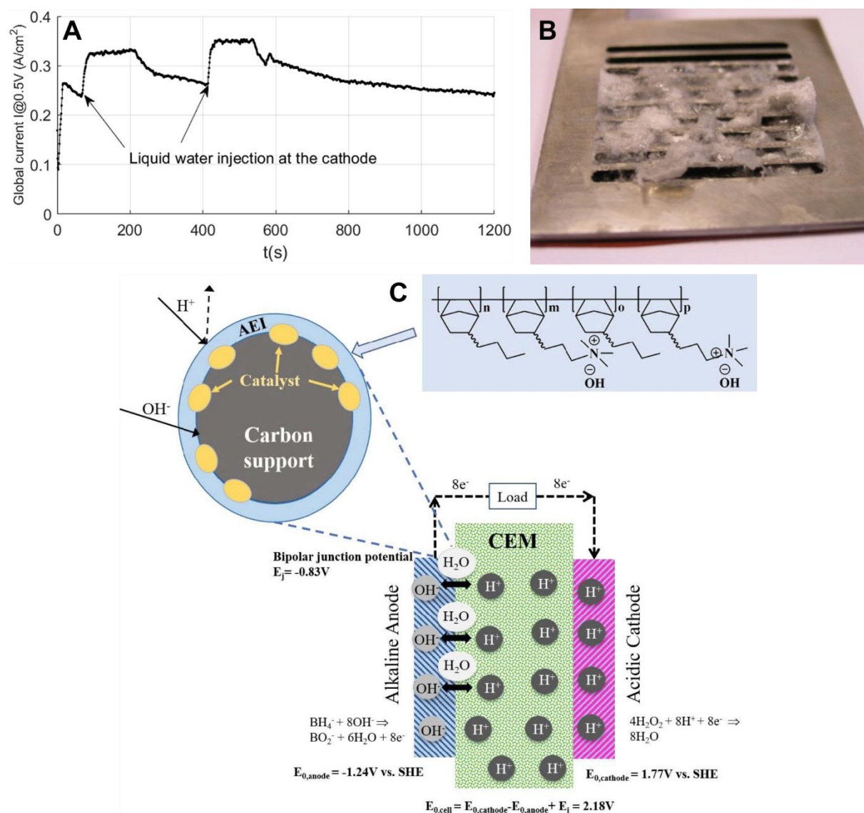
Figure 3: (A) Injection of liquid water at the cathode enables transient recovery of the performance during operation of a CEM-based DBFC at U_{\text{cell}} = 0.5\text{V} , T = 60^\circ\text{C} with a Pt/C cathode, because it washes the accumulated NaOH; reproduced from [31] with permission from Elsevier. (B) When the DBFC is operated with an anion-exchange membrane, the fuel ( \text{NaBH}_4 ) and its oxidation products ( \text{NaBO}_2 ) can be deposited in the channels of the cathode bipolar plate; reproduced from [20] with permission from Elsevier. (C) Illustration of the way a \text{H}_2\text{O}_2 -DBFC operates with pH-gradient-enabled microscale bipolar interface (BPM). Reproduced from [34] with permission from the American Chemical Society.
