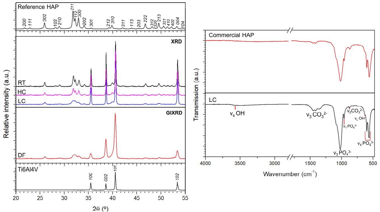
Fig. 6. (a) XRD patterns of selected as-deposited HAP coatings; samples LC, HC, and RT were measured using Bragg–Brentano geometry while grazing incidence X-ray diffraction (GIXRD) was used to characterize the thinner DF sample. (b) FTIR analysis of LC sample. For the sake of clarity, only one FTIR spectrum is shown as it is representative of all spectra obtained for HC, RT, and DF coatings.
