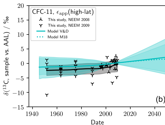
Figure D1. (a) Rayleigh plot showing observations of \delta^{13}\text{C}, \text{CFC-11} and derived \epsilon_{\text{app}}(\text{CFC-11}, \text{high-latitude}) and \epsilon_{\text{app}}(\text{CFC-11}, \text{mid-latitude}) . (b) Also shown is measured and modelled \delta_T(\text{CFC-11}) (see Fig. 4 and Sect. 2.5 for a description of the model). The model was forced with \epsilon_{\text{app}}(\text{CFC-11}, \text{high-latitude}) . The error bar in the bottom left corner of (a) shows the median repeatability of the reference gas measurements over the measurement days and the median error deriving from the fractional release factor.
