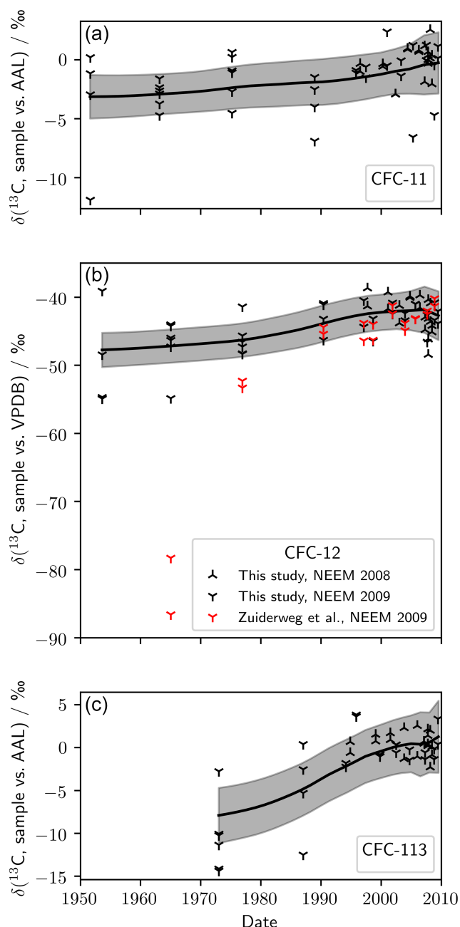
Figure 2. (a) Measured \delta(^{13}\text{C}, \text{CFC-11}) , (b) \delta(^{13}\text{C}, \text{CFC-12}) , and (c) \delta(^{13}\text{C}, \text{CFC-113}) in NEEM 2008 and 2009 firm air. Also shown is \delta(^{13}\text{C}, \text{CFC-12}) as measured by Zuiderweg et al. (2013) in the same NEEM 2009 firm air samples. The smoothed trend (black line) and 95 % confidence bounds (grey shading) were generated using a LOESS regression.
