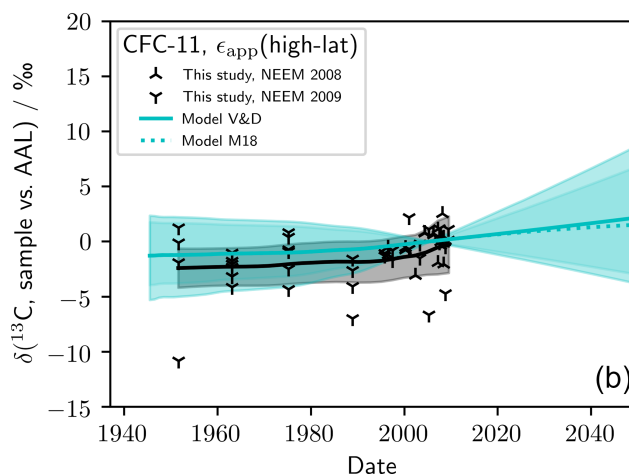
Figure D1. (a) Rayleigh plot showing observations of \delta^{13}\text{C} (CFC-11) and derived \epsilon_{\text{app}}(\text{CFC-11}, \text{high-latitude}) and \epsilon_{\text{app}}(\text{CFC-11}, \text{mid-latitude}) . (b) Also shown is measured and modelled \delta_T(\text{CFC-11}) (see Fig. 4 and Sect. 2.5 for a description of the model). The model was forced with \epsilon_{\text{app}}(\text{CFC-11}, \text{high-latitude}) . The error bar in the bottom left corner of (a) shows the median repeatability of the reference gas measurements over the measurement days and the median error deriving from the fractional release factor.
