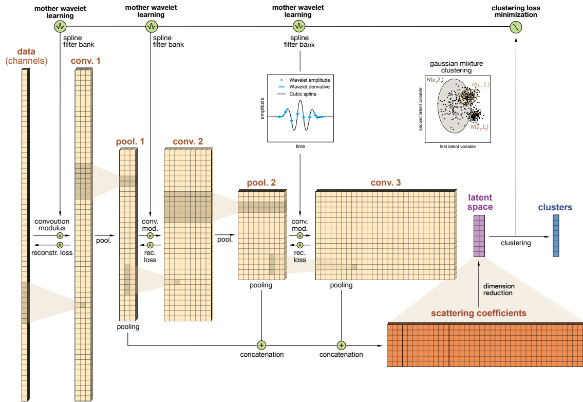
Figure 2: Deep learnable scattering network with Gaussian mixture model clustering. The network consists in a tree of convolution and modulus operations successively applied to the multichannel time series (conv1–3). A reconstruction loss is calculated at each layer in order to constrain the network not to cancel out any part of the signal (Eq. 13, Methods). From one layer to another, the convolution layers are downsampled with an average pooling operation (pool1–2), except for the last layer which can be directly used to compute the scattering coefficients. This allows to analyze large time scales of the signal structure with the increasing depth of the deep scattering network at reasonable computational cost. The scattering coefficients are finally obtained from the equal pooling and concatenation of the pool layers, forming a stable high-dimensional and multiple time and frequency scale representation of input multichannel time series. We finally apply a dimension reduction to the set of scattering coefficients obtained at each channel in order to form the low-dimensional latent space (here two-dimensional as defined in Eq. 10, Methods). We use a Gaussian mixture model in order to cluster the data in the latent space (Eq. 11, Methods). The negative log-likelihood of the clustering is used to optimize the mother wavelet at each layer (inset) with Adam stochastic gradient descent [39] described in Eq. 14 (Methods). The filter bank of each layer \ell is then obtained by interpolating the mother wavelet in the temporal domain \psi_0^{(\ell)}(t) with Hermite cubic splines (Eq. 9, Methods), and dilating it over the total number of filters J^{(\ell)}Q^{(\ell)} (Eq. 2, Methods).
