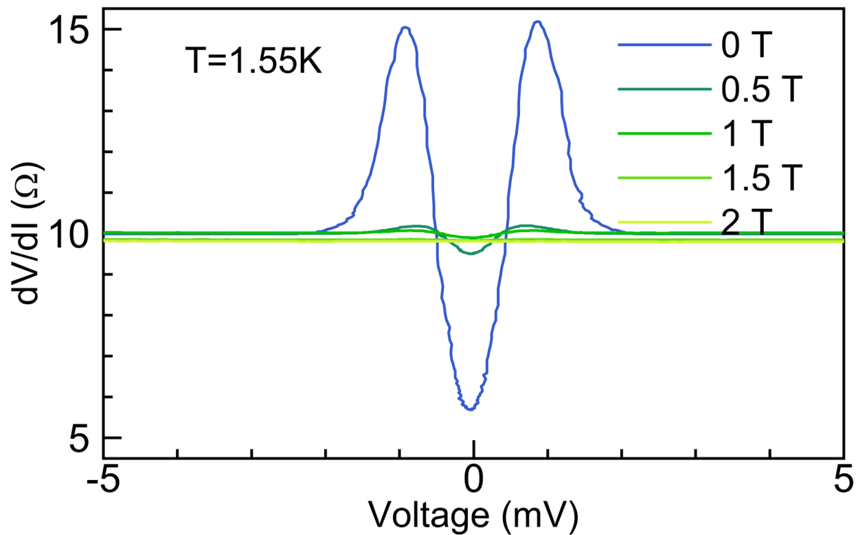
Figure 8: Differential resistance dV/dI as a function of the DC voltage in point contact measurements at different magnetic fields between 0 T and 2 T at 1.55 K, indicating the onset of the superconductivity below 1 T for T = 1.55 K.
