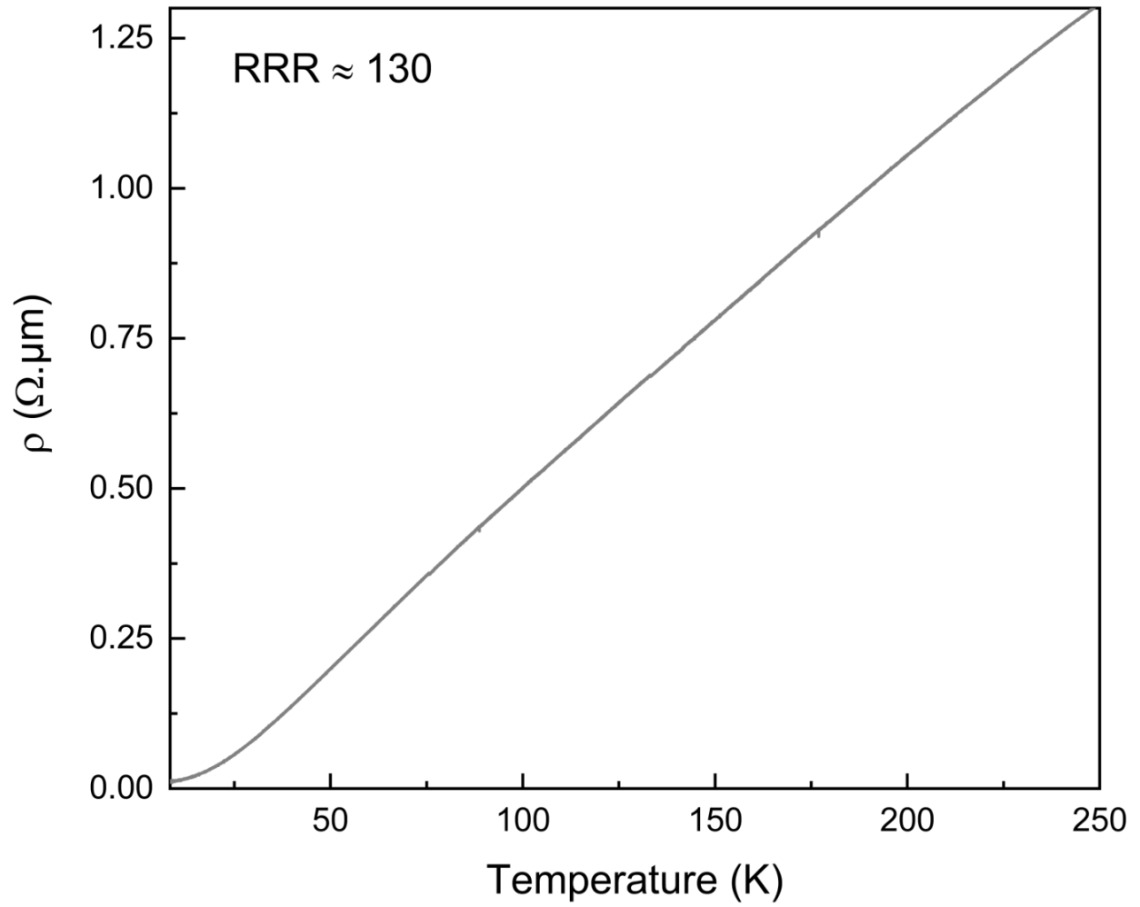
Figure 6: Temperature dependence of the resistivity of a macroscopic crystal between T = 300 K and 4.2 K.
