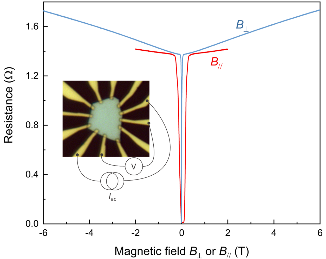
Figure 9: The magnetoresistances at T \sim 100 mK for an in-plane and out-of-plane magnetic fields are shown in red and blue respectively. A picture of the sample can be seen in the graph together with the connection configuration for the measurements of the magnetoresistances. The typical size of the sample is about 10 \mu\text{m} .
