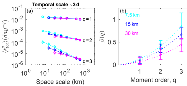
Figure 12. Spatial scaling analysis of the simulated deformation derived from the motion of triplets over a timescale of T = 3 d in three different model runs at 7.5, 15 and 30 km resolution, respectively. (a) Moments \langle \dot{\epsilon}_{\text{tot}}^q \rangle of order q = 1, 2 and 3 of the distributions of the total deformation rate \dot{\epsilon}_{\text{tot}} calculated at a temporal scale of 3 d and for spatial scales varying from 7.5 to 580 km. The solid lines indicate the associated power-law scaling \langle \dot{\epsilon}_{\text{tot}}^q \rangle \sim L^{-\beta(q)} as in Fig. 3. (b) Corresponding structure functions \beta(q) where \beta indicates the exponent of the power-law fits and q is the moment order. The bars indicate the deviation from the power law as they correspond to the minimum and maximum power-law exponents obtained for two successive spatial scales, as in Bouillon and Rampal (2015a), and thus correspond to upper-bound estimates and can be viewed as an estimation of the goodness of the fit.
