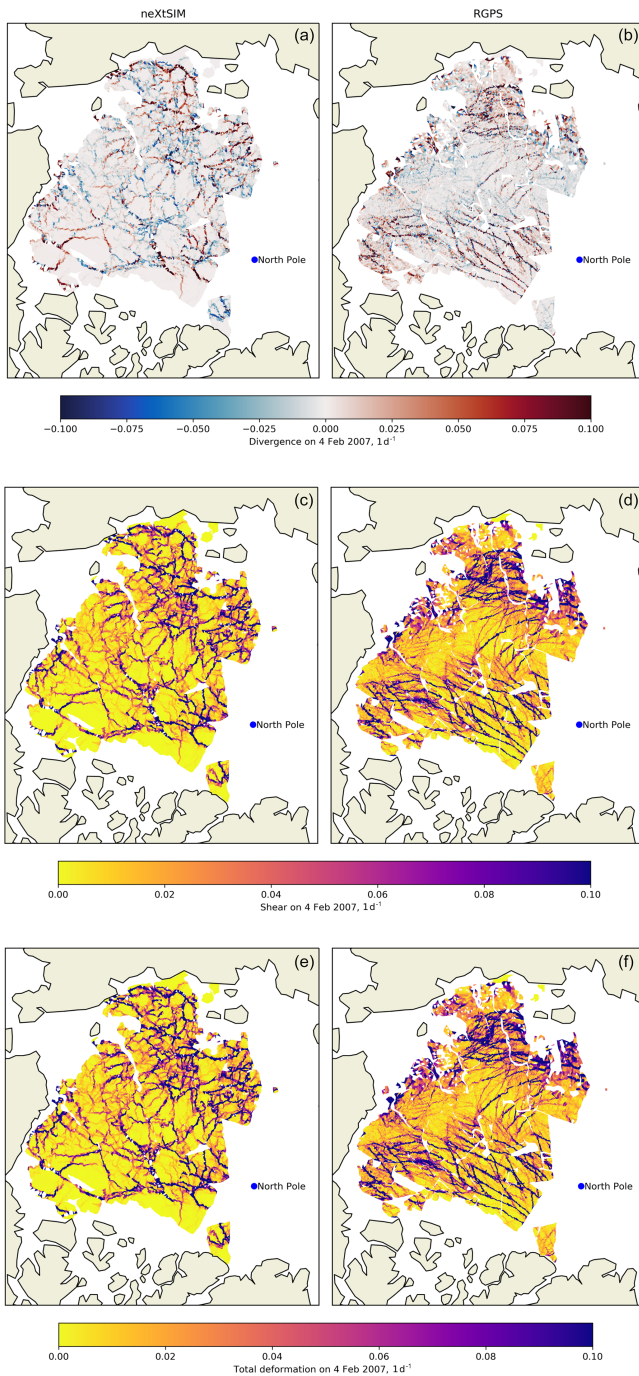
Figure 1. Divergence, shear and total sea ice deformation rates per day (top to bottom), as simulated by the model (a, c, e) and observed from satellite (b, d, f). The deformations are calculated over a timescale of 3 d. In order to get a better spatial coverage, we show all the deformation rates calculated within the period of 7 d, centered on 4 February 2007.
