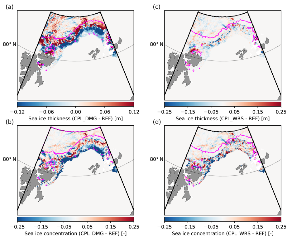
Figure 14. Snapshots of the distributions of difference in sea ice thickness ( a , c ) and sea ice concentration ( b , d ) between the CPL_DMG and the REF simulations ( a , b ) and between the CPL_WRS and REF simulations ( c , d ). All snapshots were taken on 21 October 2015 at 09:00:00 GMT. The magenta line corresponds to the contour D_{\max} = 200 m in CPL_DMG ( a , b ) and in CPL_WRS ( c , d ). The black thick lines delimit the domain used to analyse the results from the three simulations (REF, CPL_WRS, CPL_DMG) in Figs. 9, 12 and 15.
