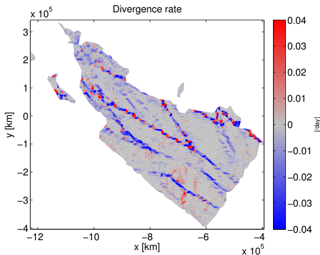
Figure 4. Unfiltered divergence rate computed from the RGPS sea ice trajectory data set and corresponding to the pair of images taken at t_{k-1} = 3 February 2007 at 17:44:00 UTC and t_k = 7 February 2007 at 17:26:35 UTC.
