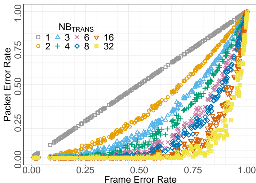
Figure 16. Experimental PER against FER for several NB_{Trans} .
