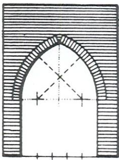
ARC OGIVAL QUINT POINT
