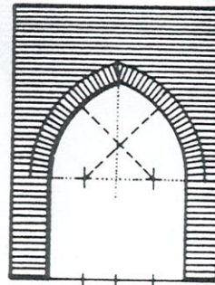
ARC OGIVAL QUART POINT
