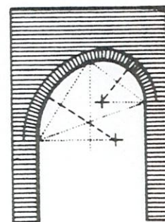
ARC RAMPANT 2 CENTRES
