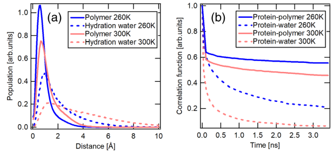
FIG. 3. (a) Displacement probability densities of polymer hydrogens (continuous lines) and hydration water (dashed lines) at 260 K (blue) and 300 K (red) after 100 ps. (b) polymer-protein (continuous lines) and water-protein (dashed lines) HB correlation function at 260 K (blue) and 300 K (red).
