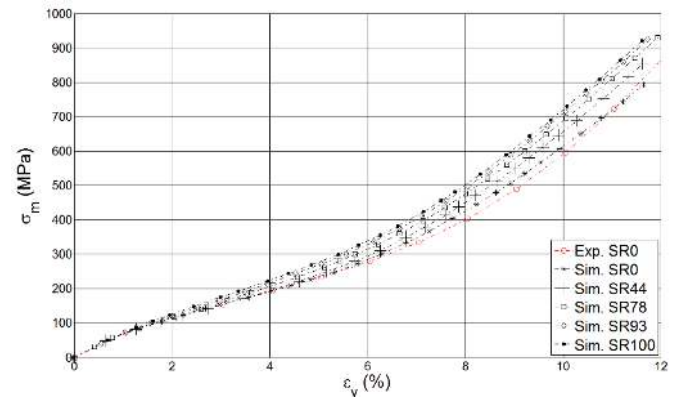
Fig. 15 Simulation of oedometric compression tests: mean stress vs. volumetric strain for different saturation ratios (Experiment S_r=0\% ; Numerical simulation S_r = 0\% , S_r = 44\% , S_r = 78\% and S_r = 100\% )
