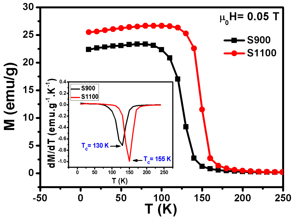
Fig. 3: Temperature dependence of magnetization and graph of dM/dT vs. T under magnetic field of \mu_0 H = 0.05 \text{ T} for S900 and S1100.
