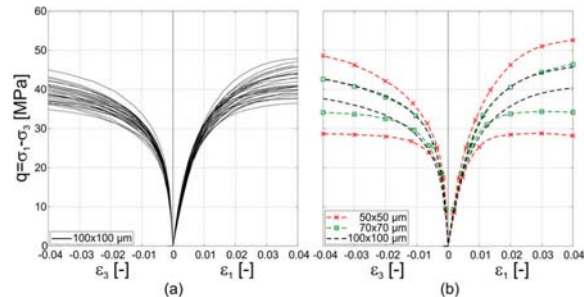
Fig. 7. Microscale response variability: to (a) randomness of EA generation and mineral contents and (b) microstructure size [11].
