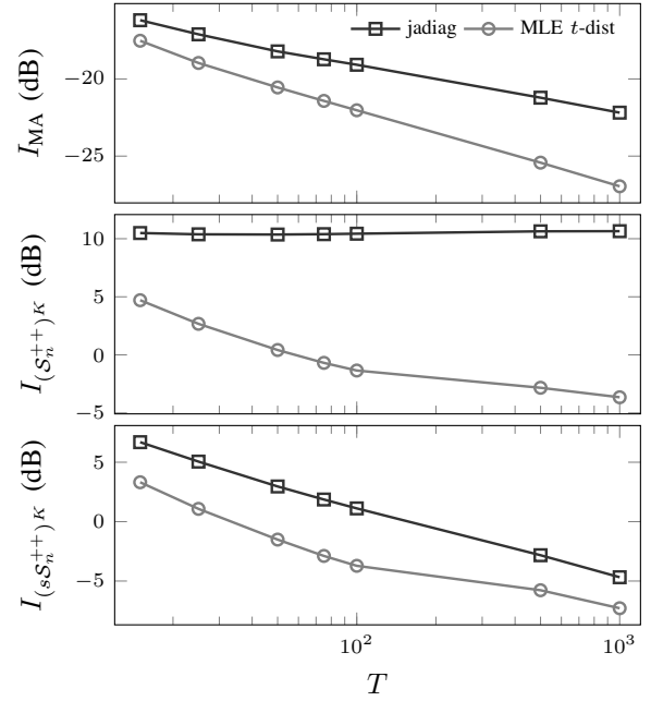
Fig. 1. Mean over 100 repetitions of the three performance indexes of the two considered blind source separation methods as functions of the number of samples T .
