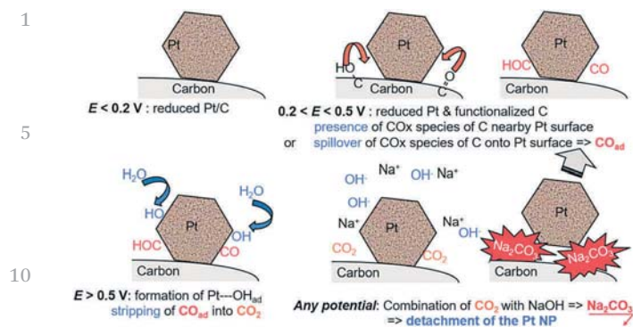
Fig. 10 Schematic representation of the processes leading to the Pt nanoparticles' detachment from their carbon support during repeated potential cycling from reducing (e.g., E = 0.1 \text{ V} vs. RHE) to oxidizing (e.g., E = 1.23 \text{ V} vs. RHE) conditions in MOH ( M = \text{Na}, \text{K}, \text{etc.} ) electrolytes with Pt/C electrocatalysts. The surface groups presented are indicative and do not pretend to be exhaustive. Freely adapted from ref. 238 with permission from Wiley.
