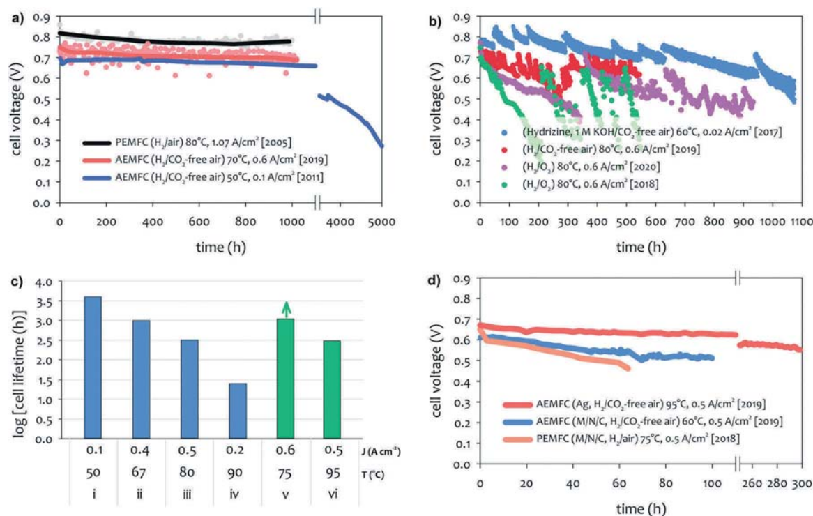
Fig. 2 AEMFC durability reported during 2017–2020 (a) durability comparison between AEMFC (2019, 74 2011 75 ) and PEMFC (2005 20 ). (b) Other significant AEMFC durability data (2017, 76 2018, 4 2019, 3 and 2020 77 ). (c) Durability of MEA's based on materials from Tokuyama Co. (blue data set) under increasingly demanding conditions of current density and temperature, compared with current results using new ionomer chemistries (green data set). Source data: (i) Fukuta 2011; 75 (ii) and (iii) PO-CellTech (unpublished data); (iv) ref. 6, ESI; (v) USC 2020 under H 2 /O 2 conditions. This cell has been operating for 1400 h as of the submission of this article with a voltage decay rate of only 7.5 \mu\text{V h}^{-1} , and the cell is still running; (vi) polyaryl-based membrane & ionomer. 6 (d) Durability of PGM-free ORR catalyzed MEAs (AEMFC (Ag), 6 AEMFC (M/N/C), 10 and PEMFC 78 ).
