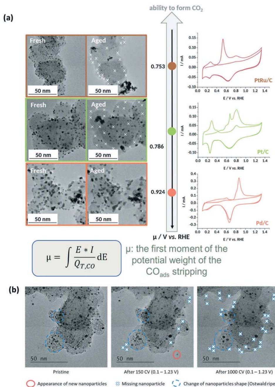
Fig. 11 (a) IL-TEM micrographs pre-AST and post-AST and CO ads stripping voltammograms recorded at \nu = 20 \text{ mV s}^{-1} in 0.1 M NaOH on 10 wt% PtRu/C (brown), 10 wt% Pt/C (green), and 10 wt% Pd/C (orange). The extent of nanoparticles detachment is correlated with the average CO ads stripping potential (first moment of the potential weight of the CO ads stripping). (b) Representative IL-TEM micrographs of Pt/C nanoparticles before (pristine) and after 150 or 1000 CV cycles performed at \nu = 100 \text{ mV s}^{-1} between 0.1 and 1.23 V vs. RHE in interface with an anion-exchange membrane in the dry cell at T = 25 \text{ }^\circ\text{C} . The markers are not comprehensive and just illustrate the main degradation mechanisms at stake during the potential cycling procedure. Reproduced from ref. 242 with permission from the American Chemical Society.
