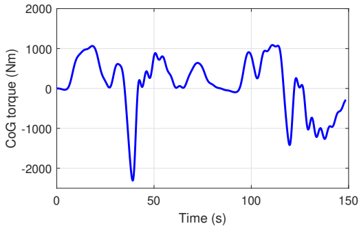
(b) Desired torque actuation
