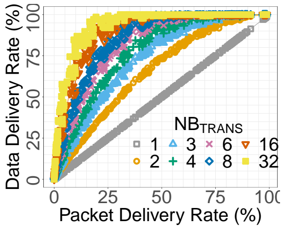
Fig. 2. Experimental DDR against PDR for several NB_{TRANS} .
