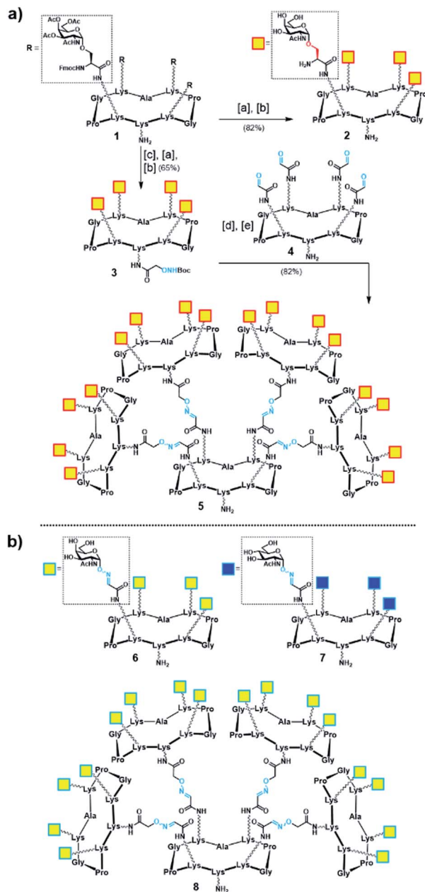
Scheme 1 (a) Synthesis of tetra- and hexadeca-valent Tn-Ser glycodendrimers 2 and 5 . Reagents and conditions: [a] 5% piperidine in \text{CH}_3\text{CN} , r.t., 15 min; [b] \text{NaOMe/MeOH} (pH \approx 10), r.t., 20 min; [c] Boc-Aoa-NHS (1.2 eq.), DIPEA (2.0 eq.), \text{CH}_3\text{CN/DMF} (1 : 1), 20 min; [d] TFA/ \text{CH}_2\text{Cl}_2 (1 : 1), r.t., 30 min; [e] 4 (ref. 72) (0.17 eq.), 0.1% TFA in \text{H}_2\text{O} , 37 °C, 45 min. (b) Tn-oxime glycodendrimers 6 (ref. 61) and 8 (ref. 73), and tetra-valent GlcNAc-oxime control 7 (ref. 73).
