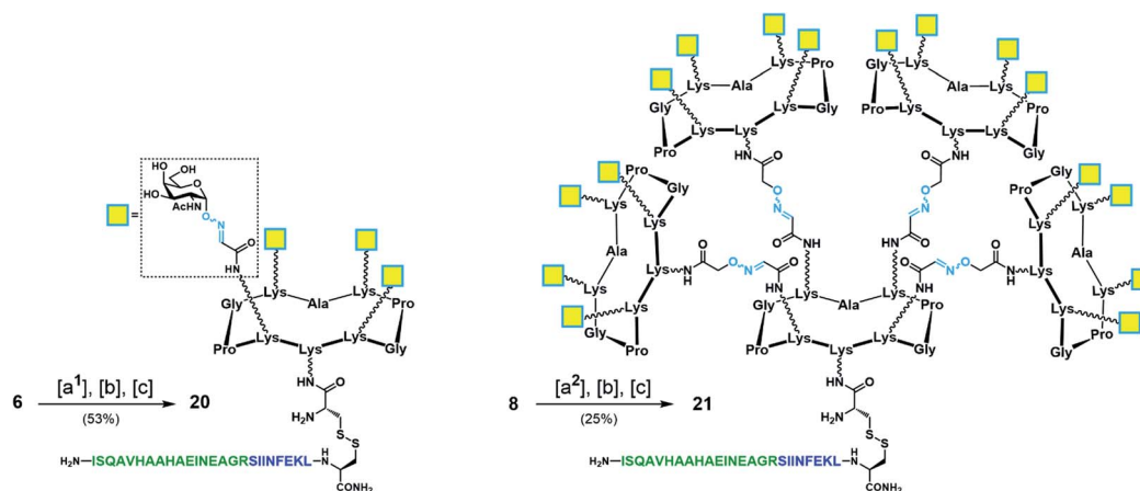
Scheme 5 Synthesis of tetravalent and hexadecavalent Tn-oxime vaccine candidates 20 and 21 . Reagents and conditions: [a 1 ] Boc-Cys(NPys)NHS (1.5–1.6 eq.), DIPEA (1.5 eq.), DMF, r.t., 30 min, 74% yield; [a 2 ] Boc-Cys(NPys)NHS (1.5 eq.), DMF/PBS (pH 7.4, 10 mM) (1 : 1), 60 min, 41% yield; [b] TFA/CH 2 Cl 2 (1 : 1), r.t., 30 min; [c] 10 (1.1–1.2 eq.), DMF/NaOAc buffer (pH 4.5, 40 mM) (1 : 1), r.t., 20 min.
