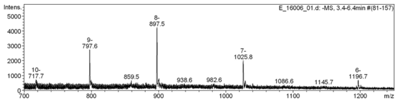
Fig. S18. ESI mass spectrum of conjugate 1
