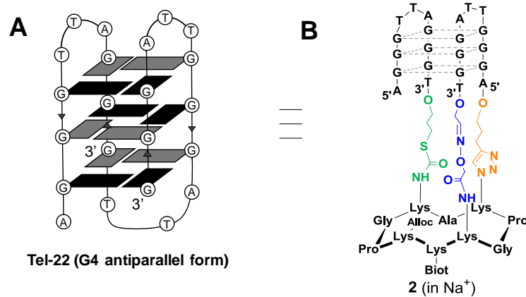
Fig. S21. A/ Schematic drawing of the G4 structure formed by the human telomeric DNA sequence (Tel-22) in presence of Na + and corresponding G-tetrad arrangements (black box = (anti) guanine, grey box = (syn) guanine B/ Schematic drawing of G4 forming DNA conjugate 2 in presence of Na +
