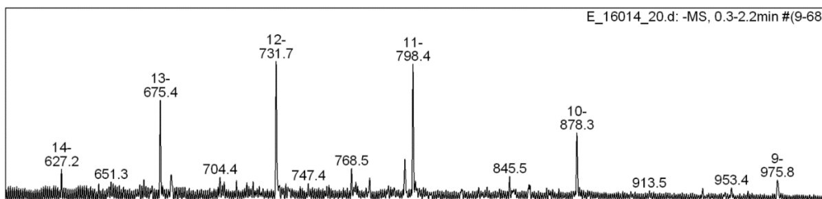
Fig. S20. ESI mass spectrum of conjugate 2
