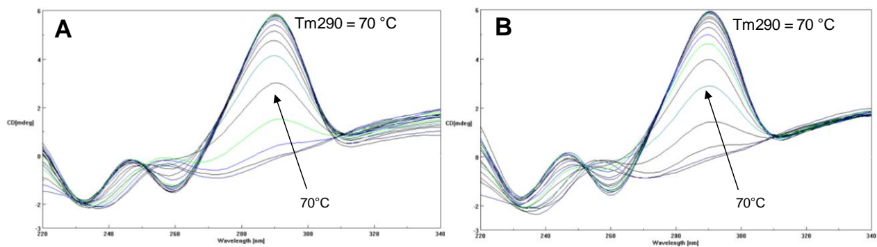
Fig. S23. Raw CD traces for 2 (3.2 \mu\text{M} in 10 mM Tris-HCl pH 7.4 with 100 mM KCl) during melting ( A , 5°C to 90°C) and annealing ( B , 90°C to 5°C).
