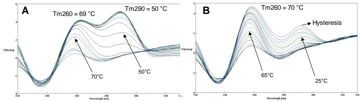
Fig. S22. Raw CD traces for 1 (3.2 \mu\text{M} in 10 mM Tris-HCl pH 7.4 with 100 mM KCl) during melting ( A , 5°C to 90°C) and annealing ( B , 90°C to 5°C).
