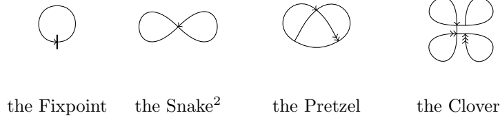
Figure 1: The self-loops
