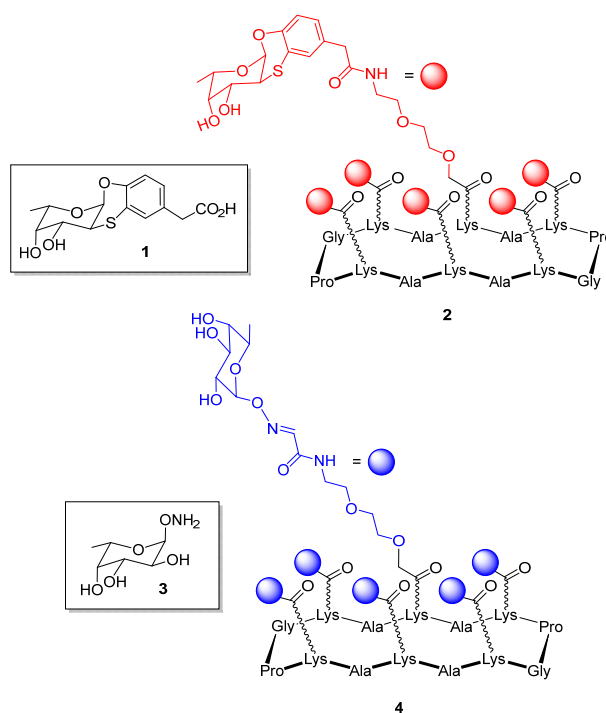
Figure 2. Structure of the aryl fucose mimetic 1 , the hexavalent conjugate 2 , the aminoxyylated fucose 3 and of the hexavalent conjugate 4 .
