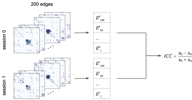
Fig. 5: The computation of ICC for global efficiency for fixed number of edges equal to 200. E_1^0, \dots, E_{100}^0, E_1^1, \dots, E_{100}^1 are values of global efficiency for each subject in both sessions; s_b is the variance between subjects, s_w is the variance within subjects in 2 sessions; ICC = (s_b - s_w)/(s_b + s_w) (see [17] for more details about computing s_b and s_w ).
