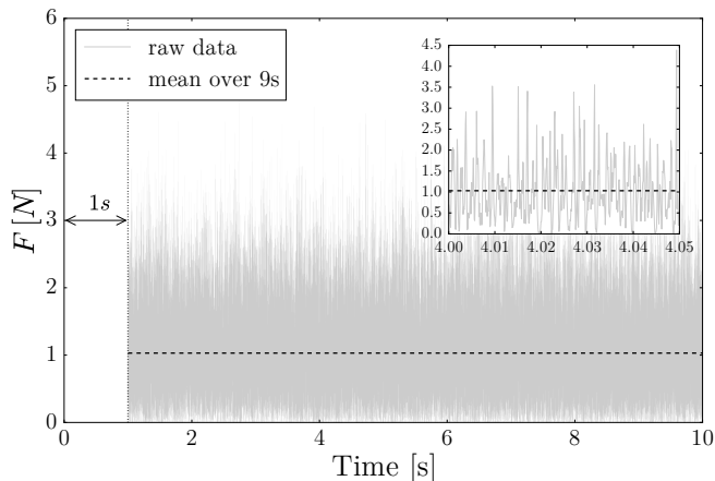
FIG. 7. Example of time-series of total force on the wall, obtained for I_M = 1.2 \cdot 10^{-2} , N_U = 10 , N_P = 25 . The instantaneous force F is highly fluctuating over time. The horizontal dashed line depicts the value of the time-averaged force, named \bar{F} , reached in the steady-state regime (after a short transient of about 1s). Inset: same data, zoomed in a time window of 0.05 s.
