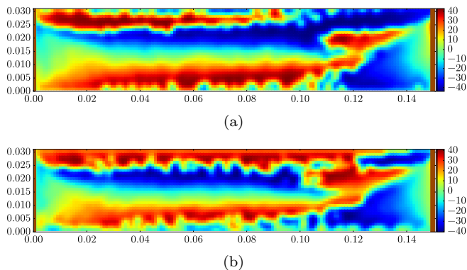
FIG. 5. Spatial maps of the principal strain (a) and stress (b) orientations averaged over time within the cavity volume: example for I_M = 6.09 \cdot 10^{-2} , N_U = 10 , N_P = 1 .
