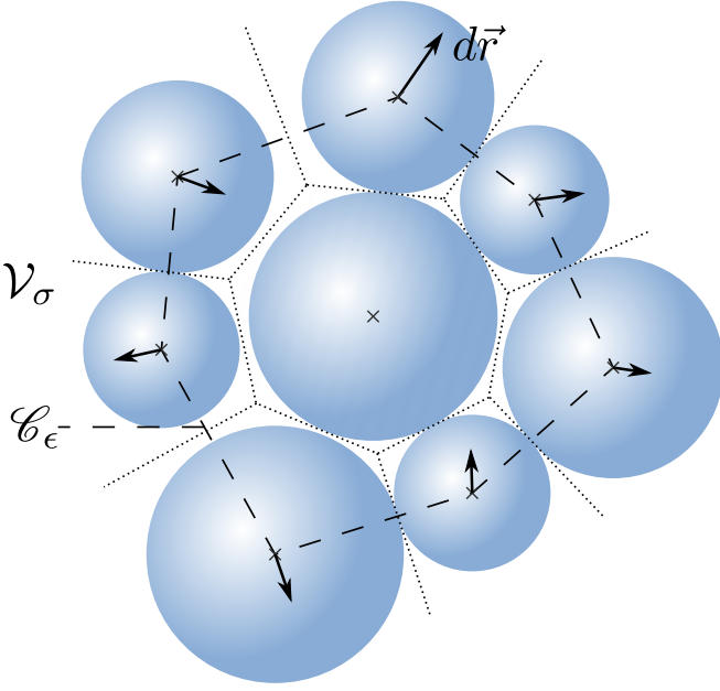
FIG. 18. Illustration of the tessellation for the per-particle volume calculation.
