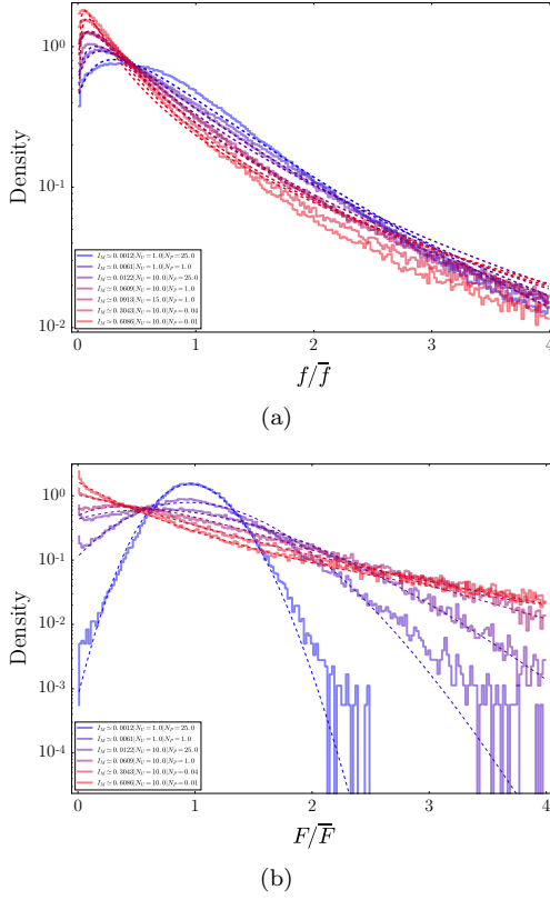
FIG. 20. Log-linear plots of the force distributions under different values of I_M for the grain-wall contact forces at particle scale (a) (see detail in caption of Fig. 12(a)) ; for the mean force on the wall (b)(see detail in caption of Fig. 13(a)).
