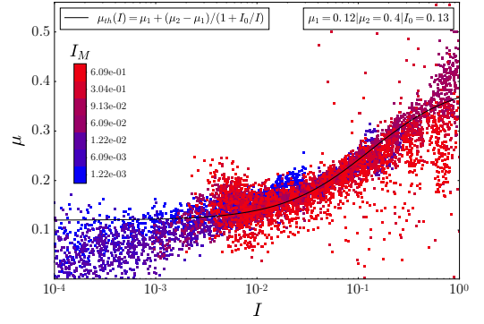
FIG. 19. Test of the local \mu(I) -rheology for all simulations of this study, including all I_M . The points come from a region of the cavity selected to approach the conditions of a simple shear flow. This region corresponds to the upper half region along y that is centered in a band of length L/2 along x .
