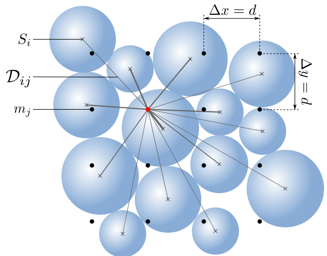
FIG. 17. Illustration of the kernel smoothing used for regular mesh fields calculations.
