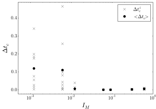
FIG. 10. Critical time \Delta t_c^i (cross symbols) beyond which the force time-series becomes weakly correlated ( C < 0.15 )—for ten portions i \in [1; 10] of the wall height, as a function of I_M . The full circles show \langle \Delta t_c \rangle that is the mean over the ten \Delta t_c^i values. The data were extracted from the autocorrelation functions plotted on Fig. 9
