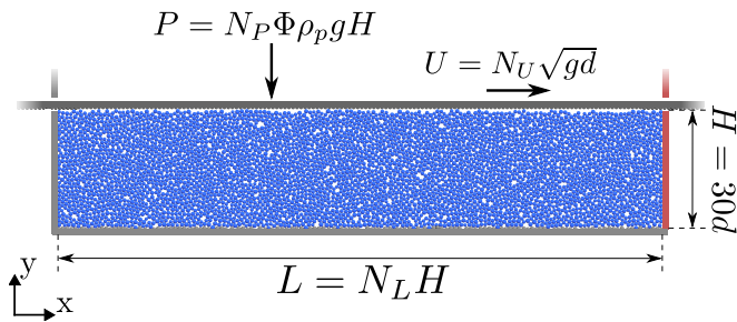
FIG. 1. Geometry and boundary conditions for the lid-driven cavity simulated by DEM. The granular sample is trapped between four walls, the top one (the lid) applies the shear displacement U and the confinement pressure P (see text for details).
