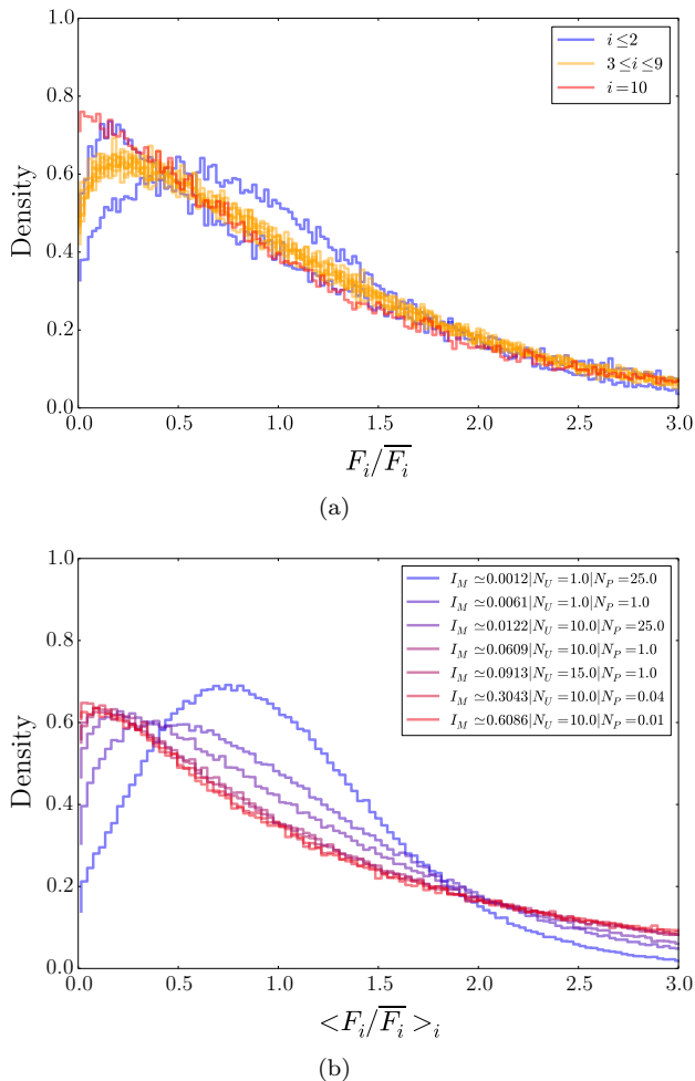
FIG. 14. (a): PDF of force time-series on ten wall portions i for I_M = 1.2 \cdot 10^{-2} , N_U = 10 , N_P = 25 (each portion time-series is scaled by its corresponding time-averaged force). The blue, orange and red curves respectively correspond to i \in [1; 2] , i \in [3; 9] and i = 10 . (b): mean distribution over i for i \in [3; 9] (yellow curves of (a)) for seven values of I_M .
