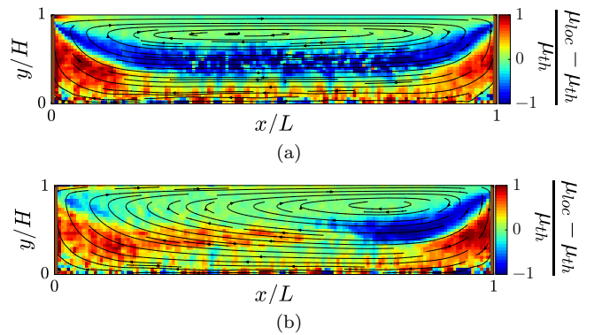
FIG. 6. Maps of (\mu_{loc} - \mu_{th})/\mu_{th} . (a): I_M = 1.22 \cdot 10^{-2} , N_U = 10 , N_P = 25 ; (b): I_M = 6.09 \cdot 10^{-2} , N_U = 10 , N_P = 1 .
