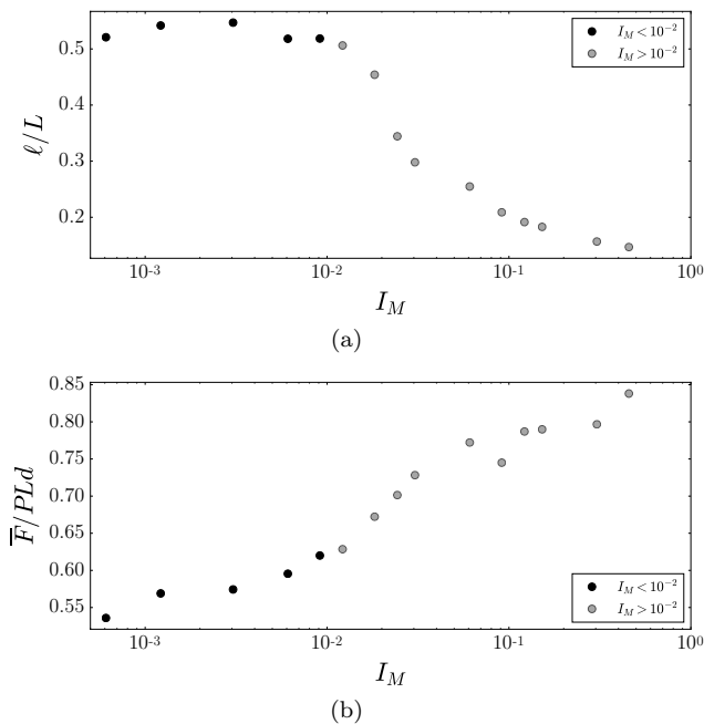
FIG. 3. (a): Distance of the vortex center from the right sidewall, \ell , relative to the cavity length L , as a function of the macroscopic inertial number I_M . (b): Mean force \bar{F} on the wall relative to the pressure force PLd imposed at the top, as a function of I_M .
