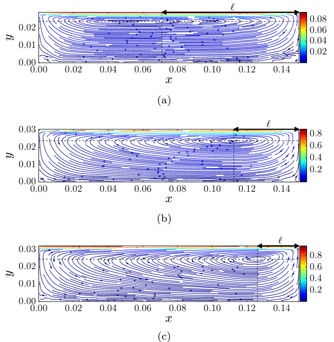
FIG. 2. Time-averaged streamlines within the cavity for three different values of I_M . (a): I_M = 1.2 \cdot 10^{-3} , N_U = 1 , N_P = 25 ; (b): I_M = 6 \cdot 10^{-2} , N_U = 10 , N_P = 1 ; (c): I_M = 0.3 , N_U = 10 , N_P = 0.04 .
