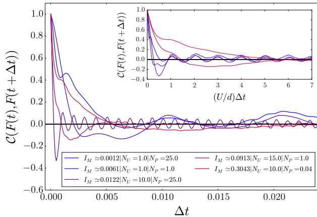
FIG. 8. Evolution of \mathcal{C}(F(t), F(t + \Delta t)) over time for five values of I_M , where F(t) is the force time-series on the entire right sidewall. Inset: \mathcal{C}(F(t), F(t + \Delta t)) plotted against (U/d)\Delta t to highlight the oscillations wavelength.
