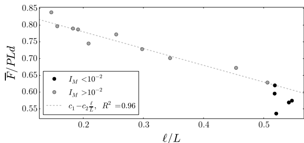
FIG. 4. \bar{F}/(PLd) versus \ell/L . The grey dashed line is a fit of Eq.(5) for I_M > 10^{-2} ( R^2 = 0.96 is the regression coefficient). This graph reveals that the mean force on the wall is entirely controlled by the distance of the vortex from the right sidewall.
