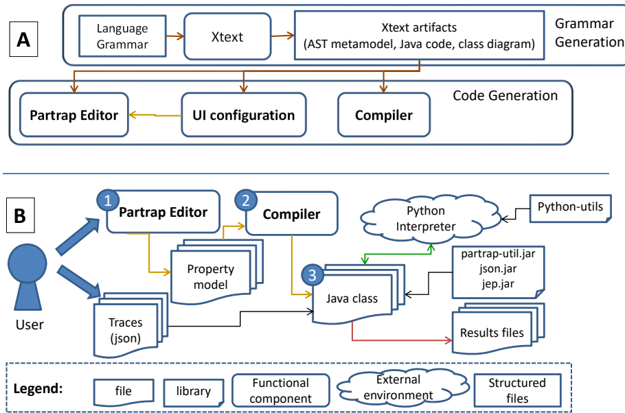
Fig. 2. Architecture of the PARTRAP toolset
