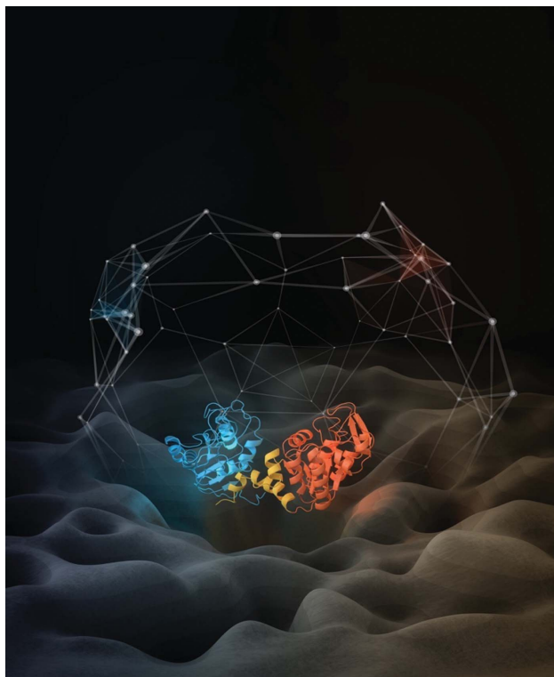
1507 1508 1509 1510 1511 1512 1513 1514 1515 1516 1517 1518 1519 1520 1521 1522 1523 1524 1525 1526 1527 1528 1529 1530 1531 1532 1533 1534 1535 Figure 6 1536 Depiction of a protein energy landscape. Protein energy landscapes can 1537 be quantitatively explored with dynamic neutron scattering. In this 1538 schematic image phosphoglycerate kinase is shown, together with an 1539 image of an energy landscape. Jumps between minima in the energy 1540 landscape can be represented by a transition matrix that can be drawn as 1541 a network. Image from https://www.scistyle.com .
