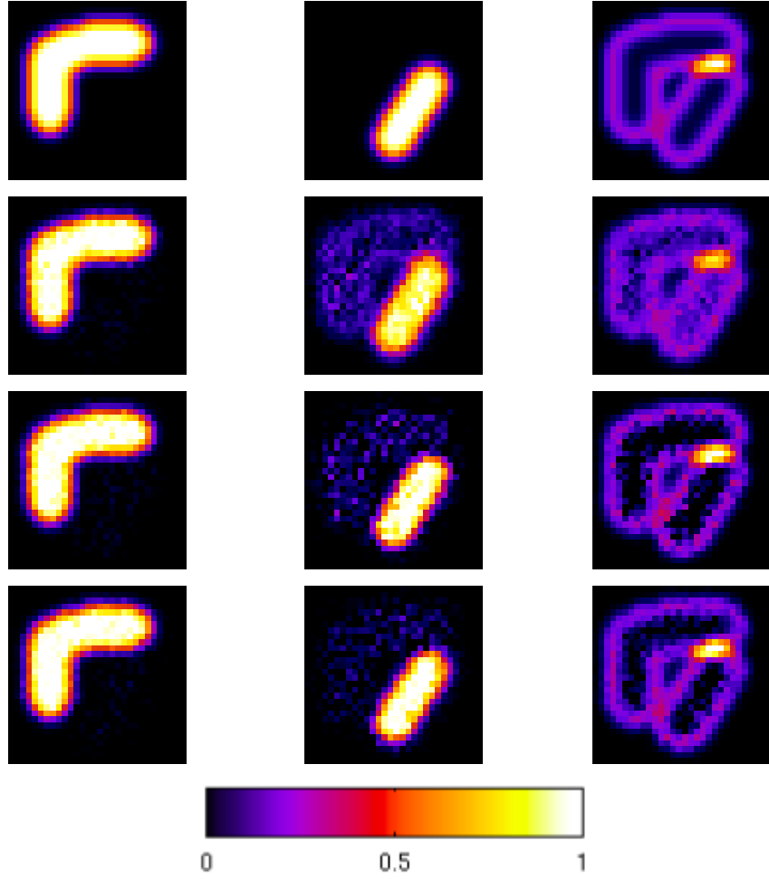
Fig. 3. Comparison of algorithms on synthetic data with a SNR of 10. First row correspond to ground truth. Row 2, 3 and 4 correspond to factor images obtained respectively with F_{REG} , F_{PLS} , F_{Global} . Column 1, 2 and 3 correspond respectively to RV, LV and myocardium.
