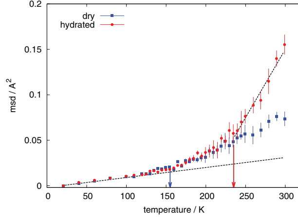
Fig. 6. – Mean squared displacements of the amino acid mixture in a D_2O -hydrated (red circles) and a dry (blue squares) state, measured on the backscattering spectrometer IN13 ( 8\mu\text{eV} resolution, ILL, Grenoble). Experimental error bars are indicated as vertical lines. Blue and red arrows indicate the temperature regions of the two main anharmonic onsets.
