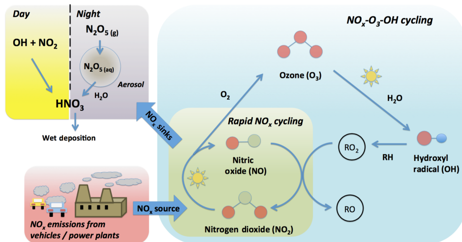
Figure 1. Schematic of the \text{NO}_x\text{-O}_3\text{-OH} relationship in the background troposphere.
