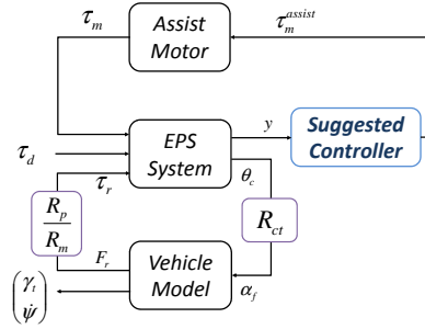
Fig. 10. Simulation structure for the suggested control strategy
