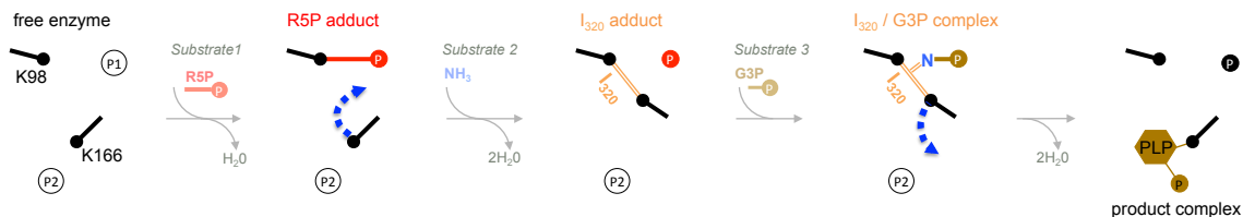
Figure 4 | The central role of I 320 intermediate transfer in vitamin B6 biosynthesis. a,
