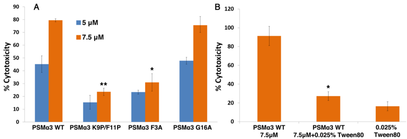
Fig. 3. PSM \alpha 3 toxicity against human T-cells is dependent on its ability to form fibrils.
