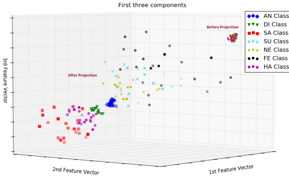
Figure 5: Data distribution before and after projection.
