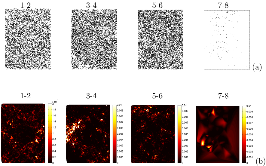
Figure 21: Spatial distribution of c- contacts (a), and field of intensity of w_2^c for c- contacts, for the proportional strain loading path applied on sample MD for R = 0.8 ; numbered snapshots are identified in Fig. 7c.
