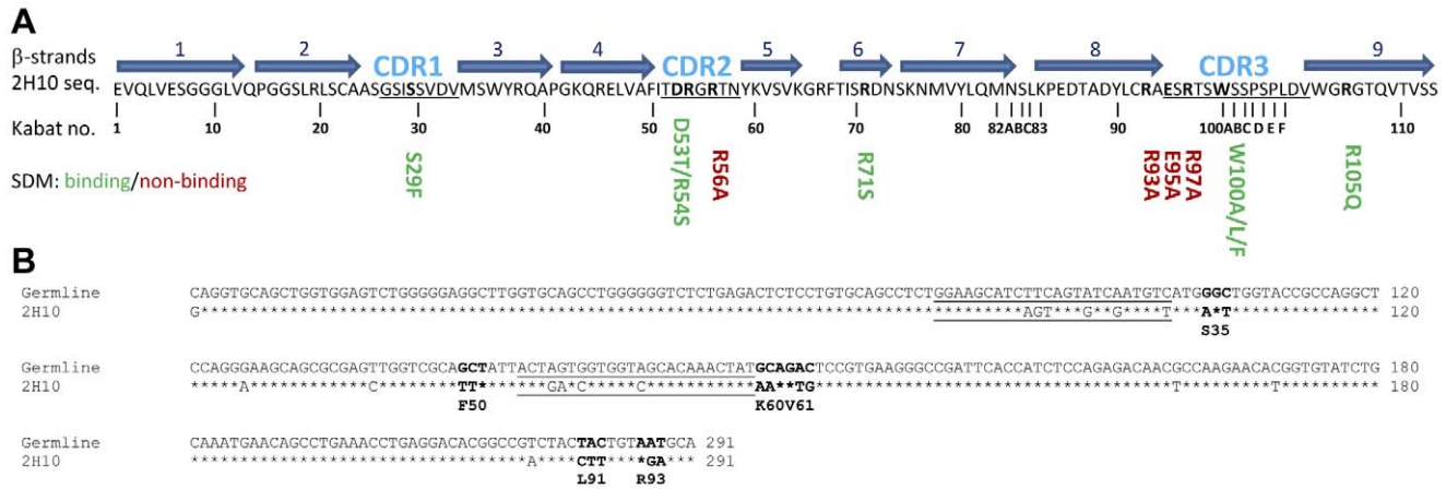
Figure 2. Amino acid and DNA sequence of 2H10. A ) Amino acid sequence. Secondary structure assignment is based on the crystal structure. \beta -strands are depicted as blue arrows. CDR regions are indicated with CDR1 to CDR3 and are underlined. Residues depicted in bold were mutated. Mutants that still showed binding are shown in green and mutants that do not bind to the antigen anymore are shown in red. B ) DNA sequence alignment of 2H10 with the germline V-gene from which it originated. The asterisks indicate identical nucleotides. The CDR1 and CDR2 coding regions are underlined. Codons with at least two point mutations are in boldface. doi:10.1371/journal.ppat.1003202.g002
