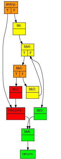
(c) Colored cfg for FAILURE not to be reached
