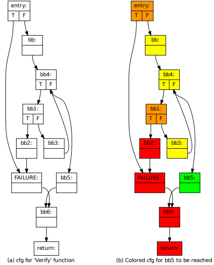
(a) cfg for Verify function (b) Colored cfg for bb5 to be reached
